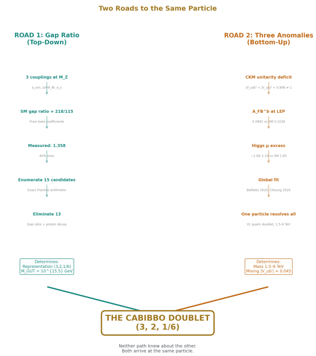
Figure 2: Fig. 2: The gap ratio path (top-down: 3 couplings → enumeration → elimination) and the anomaly path (bottom-up: CKM deficit + A_FB^b + Higgs \mu → global fit) converge independently on (3,2,1/6).
