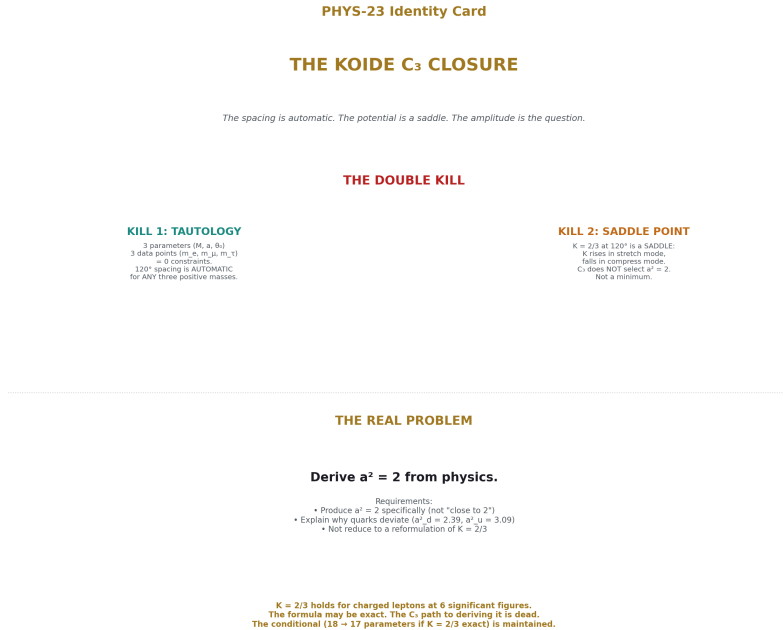
Figure 8: Fig. 8: Double kill — tautology (3 params, 3 masses, 0 constraints) + saddle ( K rises and falls from 2/3 ). The real problem: derive a^2 = 2 . The conditional 18 \rightarrow 17 is maintained, not resolved.
