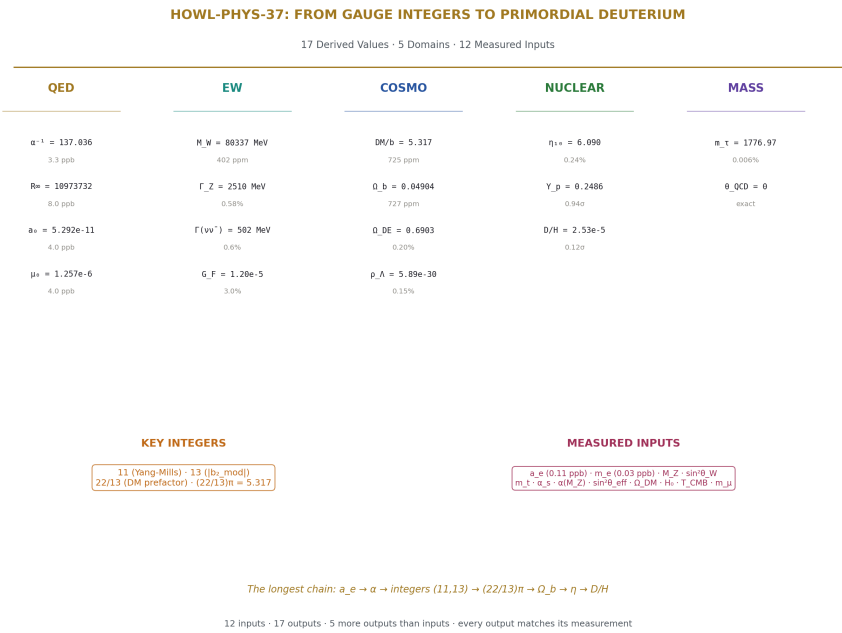
Figure 1: Fig. 8: Identity card — 17 derived values across QED, electroweak, cosmology, nuclear, and mass domains from 12 measured inputs.
