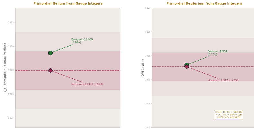
Figure 4: Fig. 5: Primordial helium (0.94σ) and deuterium (0.12σ) predicted from gauge integers — both within measurement uncertainties.
