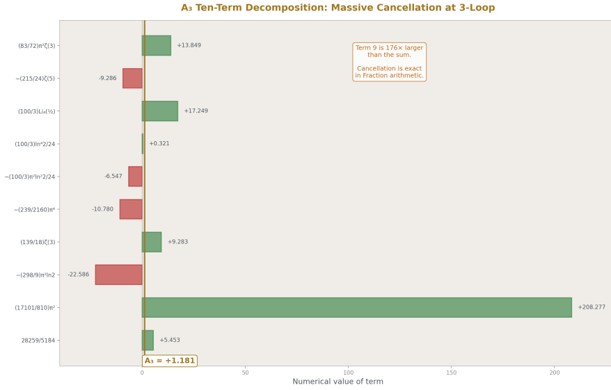
Figure 3: Fig. 5: The ten terms of A_3 span -23 to +208, cancelling to +1.181 — a 176 \times cancellation exact in Fraction arithmetic.
