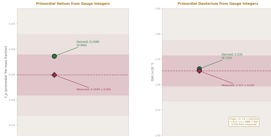
Figure 4: Fig. 5: Primordial helium (0.94σ) and deuterium (0.12σ) predicted from gauge integers — both within measurement uncertainties.
