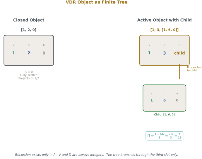
Figure 2: Fig. 6: VDR Tree Structure — Closed object [1,2,0] vs active object [1,3,[1,6,0]] showing recursion through R only.
