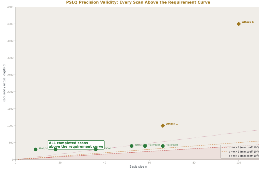
Figure 2: Fig. 7: Every completed PSLQ scan (green dots) sits above the theoretical precision requirement curve. All null results are mathematically valid. Future attacks (gold diamonds) have even larger margins.
