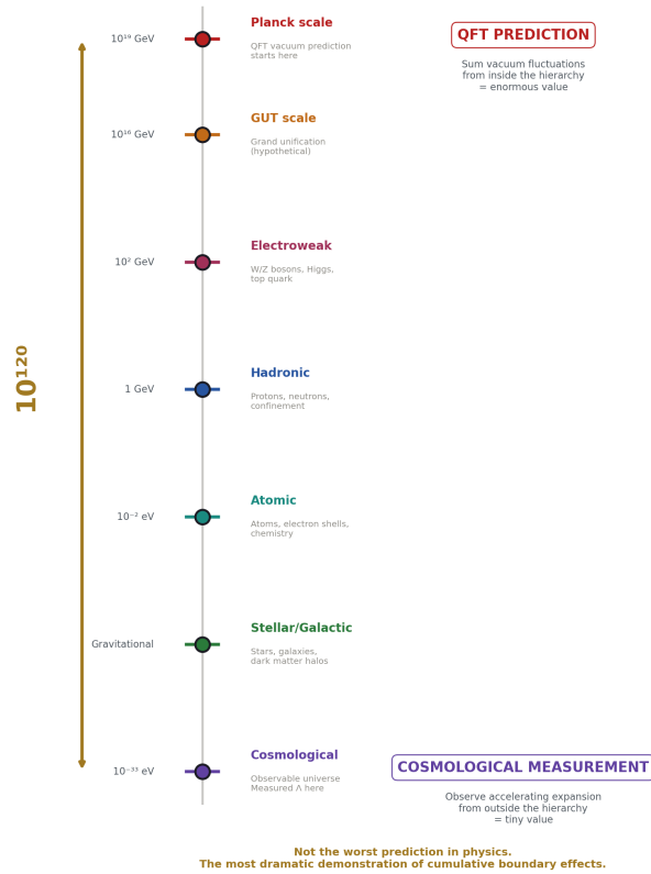
Figure 7: Fig. 3: From Planck scale to cosmological scale — the 10^{120} discrepancy spans the entire boundary hierarchy, every coherent structure layer between the two measurements.
