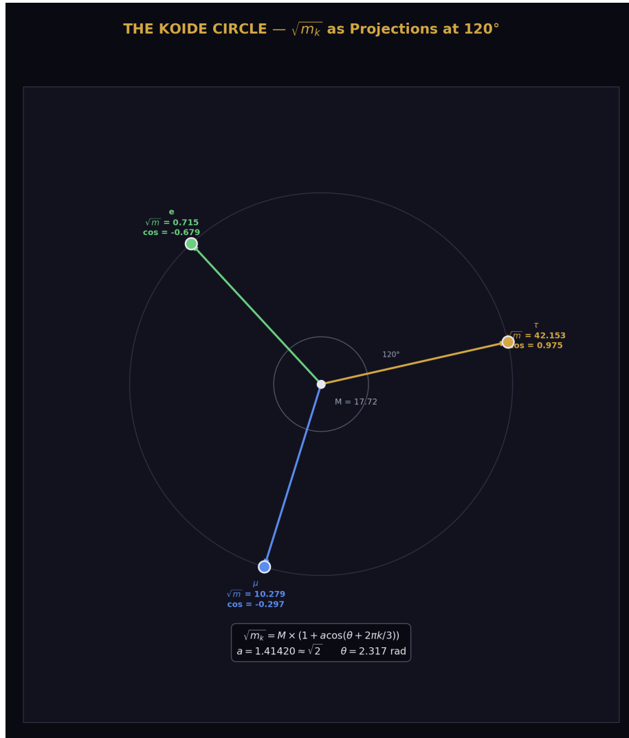
Figure 2: Fig. 2: The Koide parametrization visualized as projections of three vectors at 120^\circ separation on a circle of radius a \approx \sqrt{2} .
