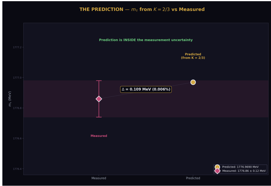
Figure 7: Fig. 6: Zoomed view of the m_\tau prediction (1776.97 MeV) vs measurement ( 1776.86 \pm 0.12 MeV). The prediction falls inside the 1\sigma measurement band.
