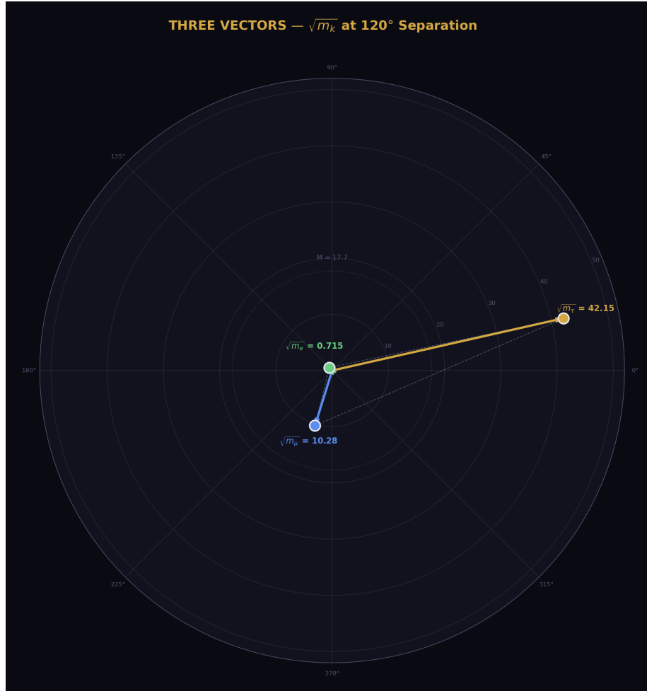
Figure 3: Fig. 8: The three \sqrt{m} vectors on a polar plot at 120^\circ separation. The tau vector dominates, the electron vector is near the origin, and the M = 17.7 circle marks the equal-mass reference.
