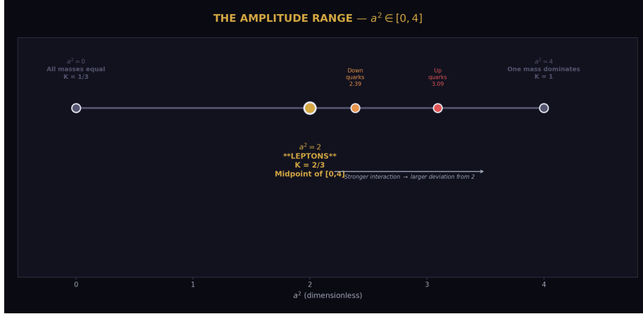
Figure 4: Fig. 5: The allowed range a^2 \in [0,4] showing the lepton value at the geometric midpoint a^2 = 2 , with quark sectors displaced toward stronger interaction.
