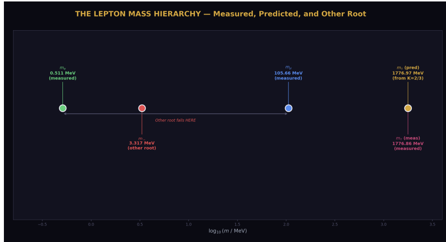
Figure 6: Fig. 4: The charged lepton masses on a log scale with the Koide prediction (gold) at the measured tau position and the other quadratic root (red) between electron and muon.
