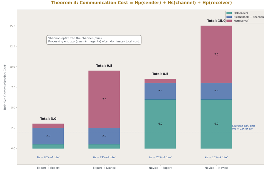
Figure 7: Fig. 8: Communication Cost Composition — Total cost decomposed into H_p(\text{sender}) + H_s(\text{channel}) + H_p(\text{receiver}) across four scenarios. Shannon's channel cost (blue) is constant; processing entropy (cyan, magenta) dominates in expert-novice communication.
