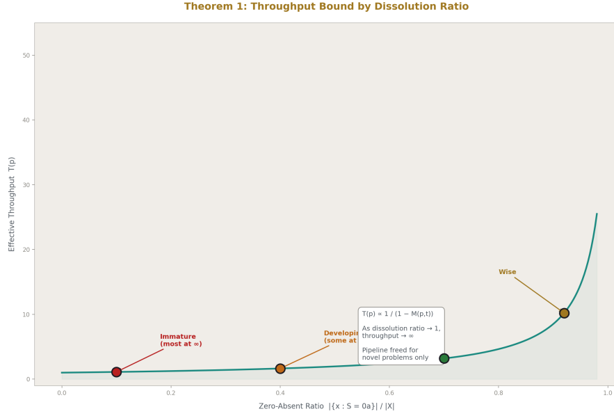
Figure 8: Fig. 4: Throughput Bound — Effective throughput increases nonlinearly as the zero-absent ratio grows. Maturity stages marked: immature systems saturated, wise systems operating with freed pipeline.
