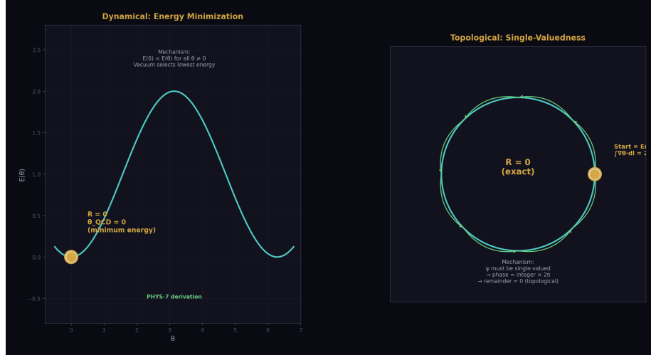
Figure 4: Fig. 2: Energy minimization gives \theta_{QCD}=0 (dynamical, left). Wavefunction single-valuedness gives flux quantization (topological, right). Same result R=0 , different physics.
