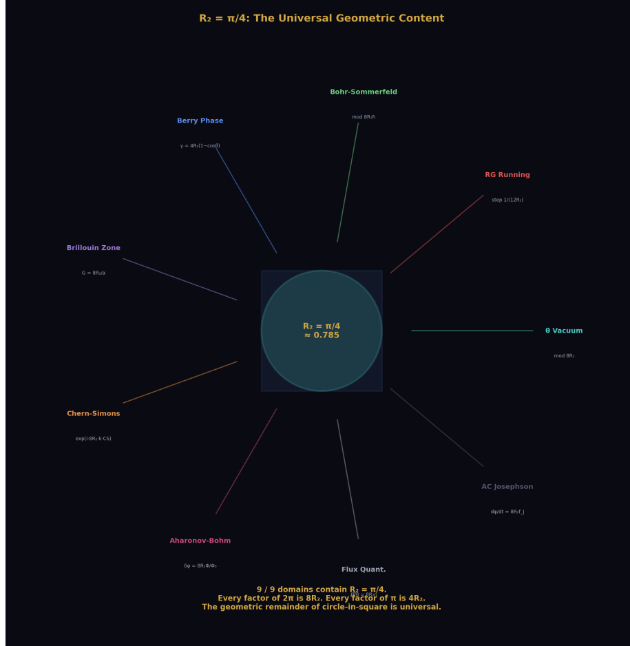
Figure 7: Fig. 4: The circle inscribed in its bounding square ( R_2 = \pi/4 ) radiating to all nine physics domains — every factor of 2\pi is 8R_2 , present in 9/9 domains.
