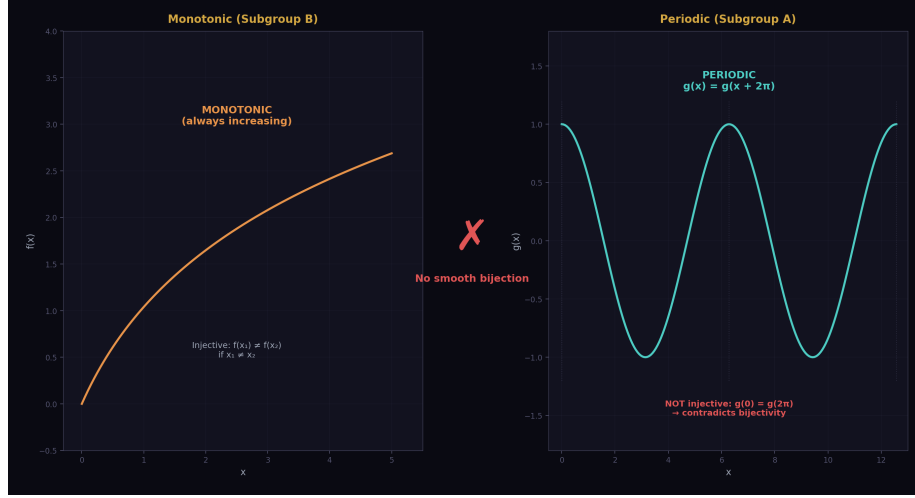
Figure 6: Fig. 7: A monotonic function (injective, always increasing) cannot be mapped to a periodic function (not injective) by any smooth bijection — the three-subgroup classification is topological.
