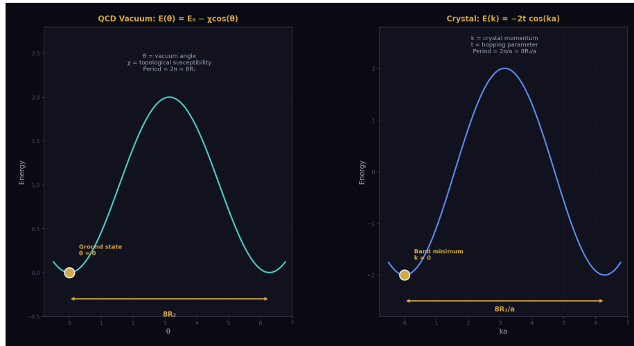
Figure 3: Fig. 3: E(\theta) = E_0 - \chi \cos(\theta) and E(k) = -2t \cos(ka) — the same mathematics (cosine on 8R_2 domain, minimum at 0) describing vacuum topology and crystal band structure.
