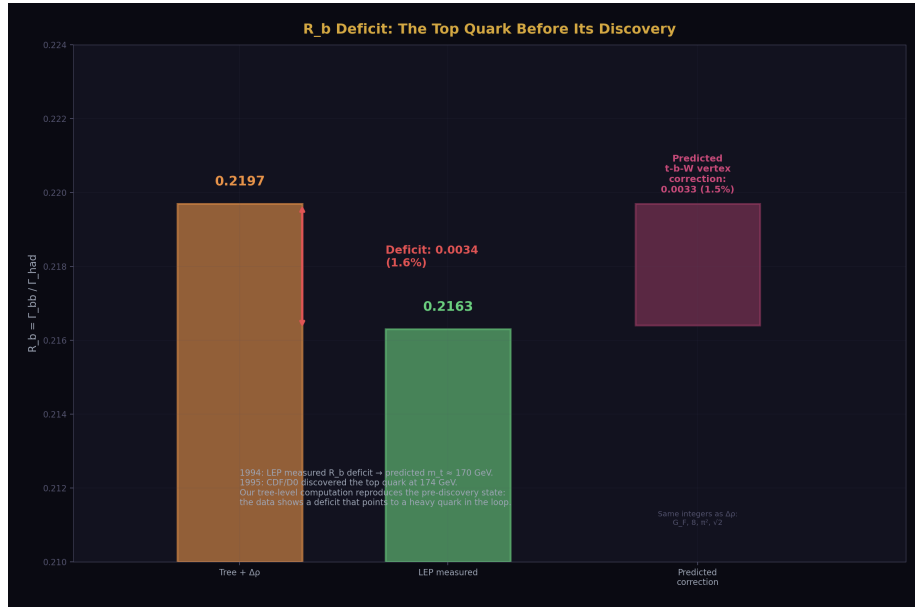
Figure 4: Fig. 6: R_b computed (0.2197) vs measured (0.2163) — the 1.6% deficit matches the predicted 1.5% t-b-W vertex correction, reproducing the 1994 evidence that predicted the top quark.
