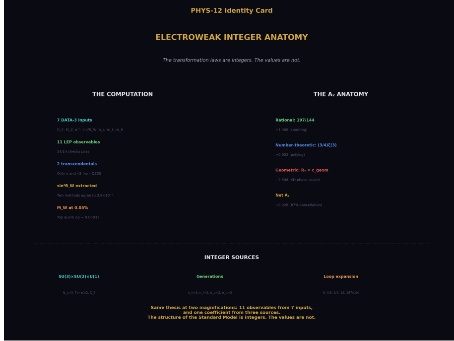
Figure 8: Fig. 8: 11 LEP observables from 7 inputs with only \pi and \sqrt{2} as transcendentals, A_2 decomposed into rational + \zeta(3) + R_4 with 87% cancellation — the integer anatomy at two magnifications.
