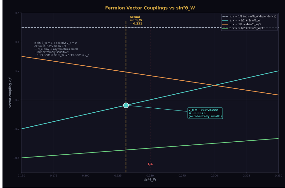
Figure 1: Fig. 1: Four fermion vector couplings as functions of \sin^2\theta_W — the electron coupling crosses zero near 1/4 , making v_e accidentally small and asymmetries extremely sensitive.
