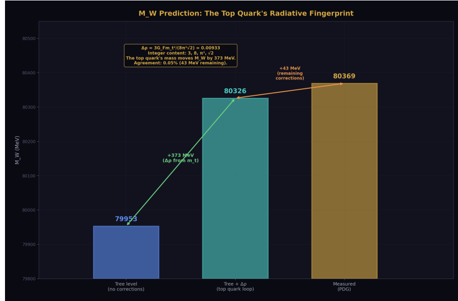
Figure 2: Fig. 5: M_W goes from 79953 (tree) to 80326 (tree+ \Delta \rho ) to 80369 (measured) — the \Delta \rho correction from the top quark mass closes 90% of the gap with integer content 3, 8, \pi^2 , \sqrt{2} .
