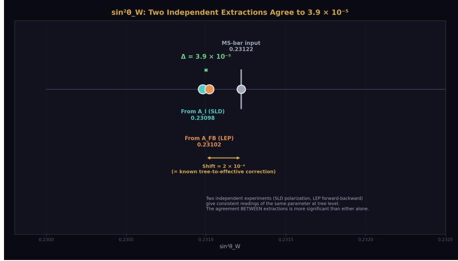
Figure 5: Fig. 4: \sin^2\theta_W extracted from A_1 (SLD: 0.23098) and A_{FB} (LEP: 0.23102) agree to 3.9 \times 10^{-5} — two independent experiments give consistent readings, both shifted by the known tree-to-effective correction.
