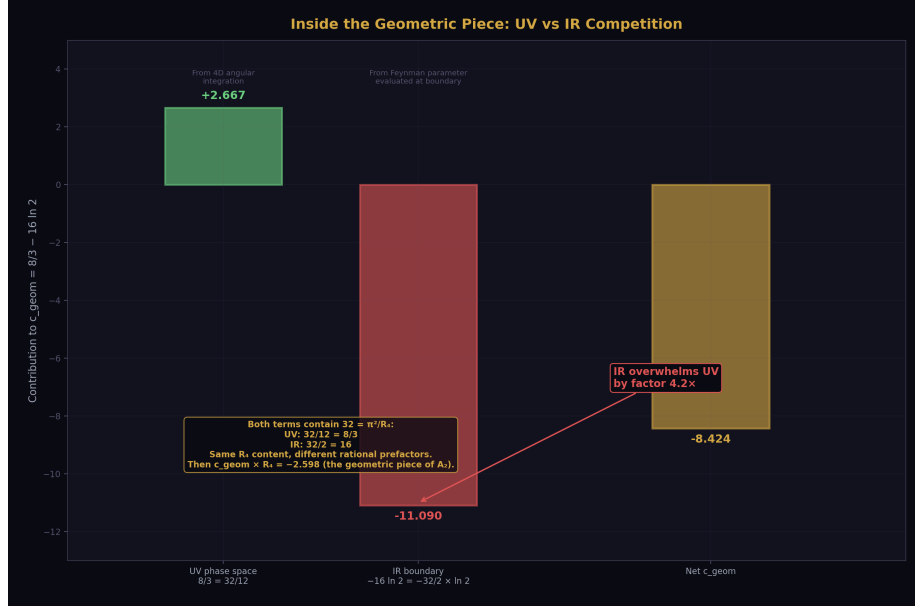
Figure 7: Fig. 7: Within c_{\text{geom}} = 8/3 - 16 \ln 2 , the UV phase space (+2.667) competes with IR boundary (-11.090) — IR overwhelms UV by 4.2 \times , both containing the same R_4 = \pi^2/32 with different rational prefactors.
