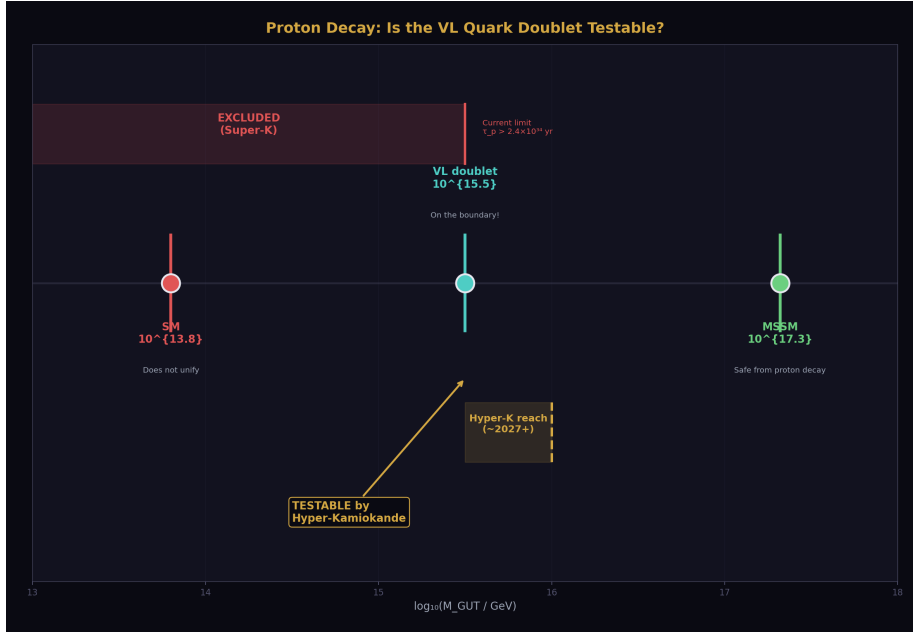
Figure 6: Fig. 2: M_{\text{GUT}} for SM ( 10^{13.8} ), VL doublet ( 10^{15.5} ), and MSSM ( 10^{17.3} ) vs the Super-K exclusion and Hyper-K projected reach — the VL doublet sits on the testable boundary.
