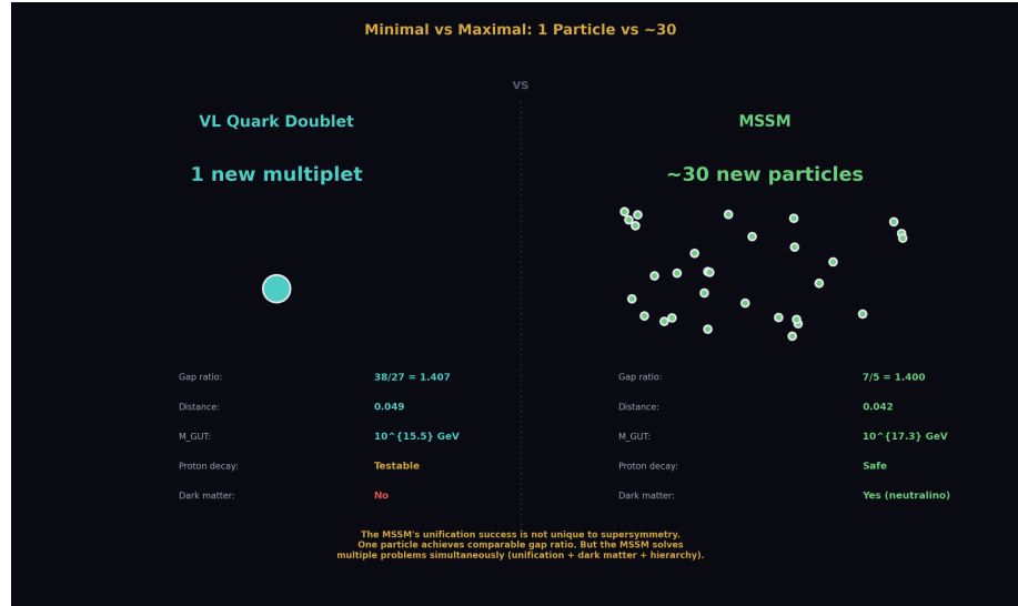
Figure 7: Fig. 6: The VL quark doublet (1 new particle) achieves gap ratio 38/27 , comparable to the MSSM ( \sim 30 particles) at 7/5 — the MSSM's unification success is not unique to supersymmetry.
