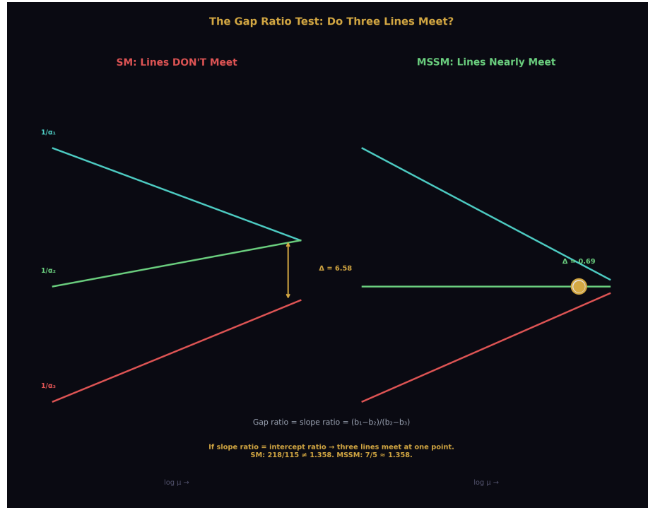
Figure 2: Fig. 5: Unification as a three-line convergence test — the gap ratio is the slope ratio. If it matches the intercept ratio, the lines meet. SM: they don't. MSSM: they nearly do.
