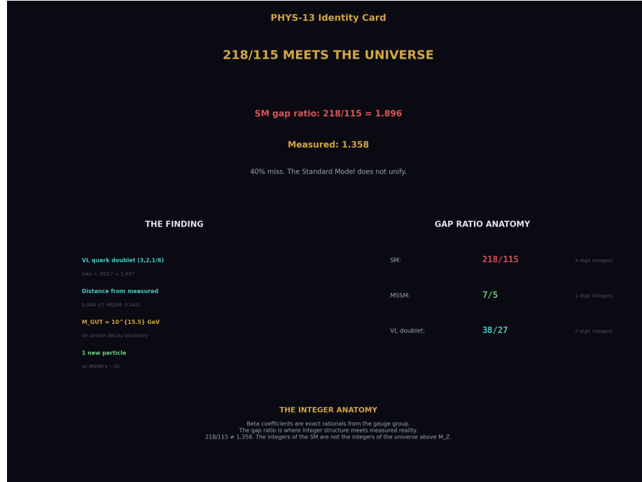
Figure 8: Fig. 8: 218/115 meets the universe — SM fails by 40%, VL quark doublet and MSSM succeed to ~3%, beta coefficients are exact rationals from the gauge group.
