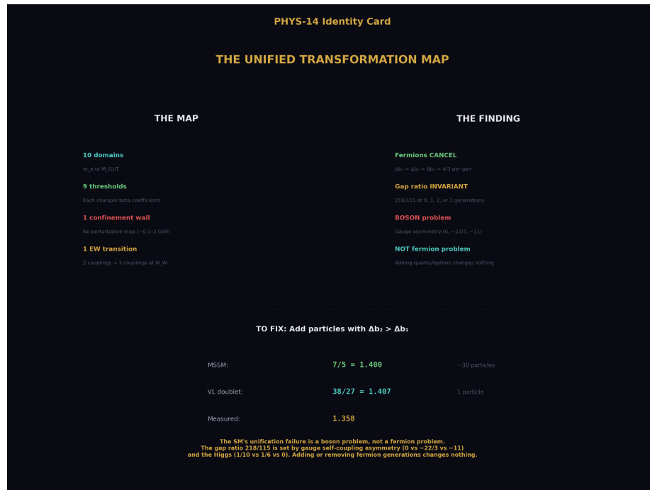
Figure 8: Fig. 8: 10 domains, fermion cancellation ( \Delta b_1 = \Delta b_2 = \Delta b_3 = 4/3 ), boson problem (gauge asymmetry sets 218/115), fix requires asymmetric BSM content (VL doublet or MSSM).
