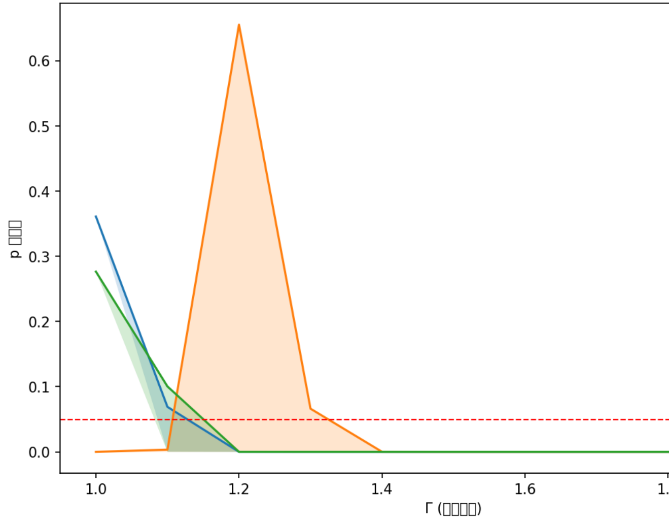
Rosenbaum \gamma vs p
