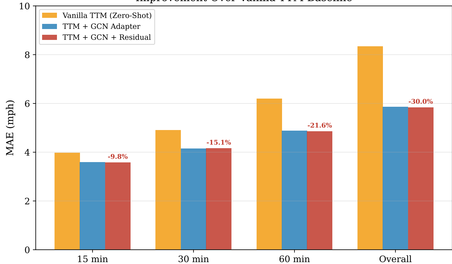
Improvement Over Vanilla TTM Baseline
