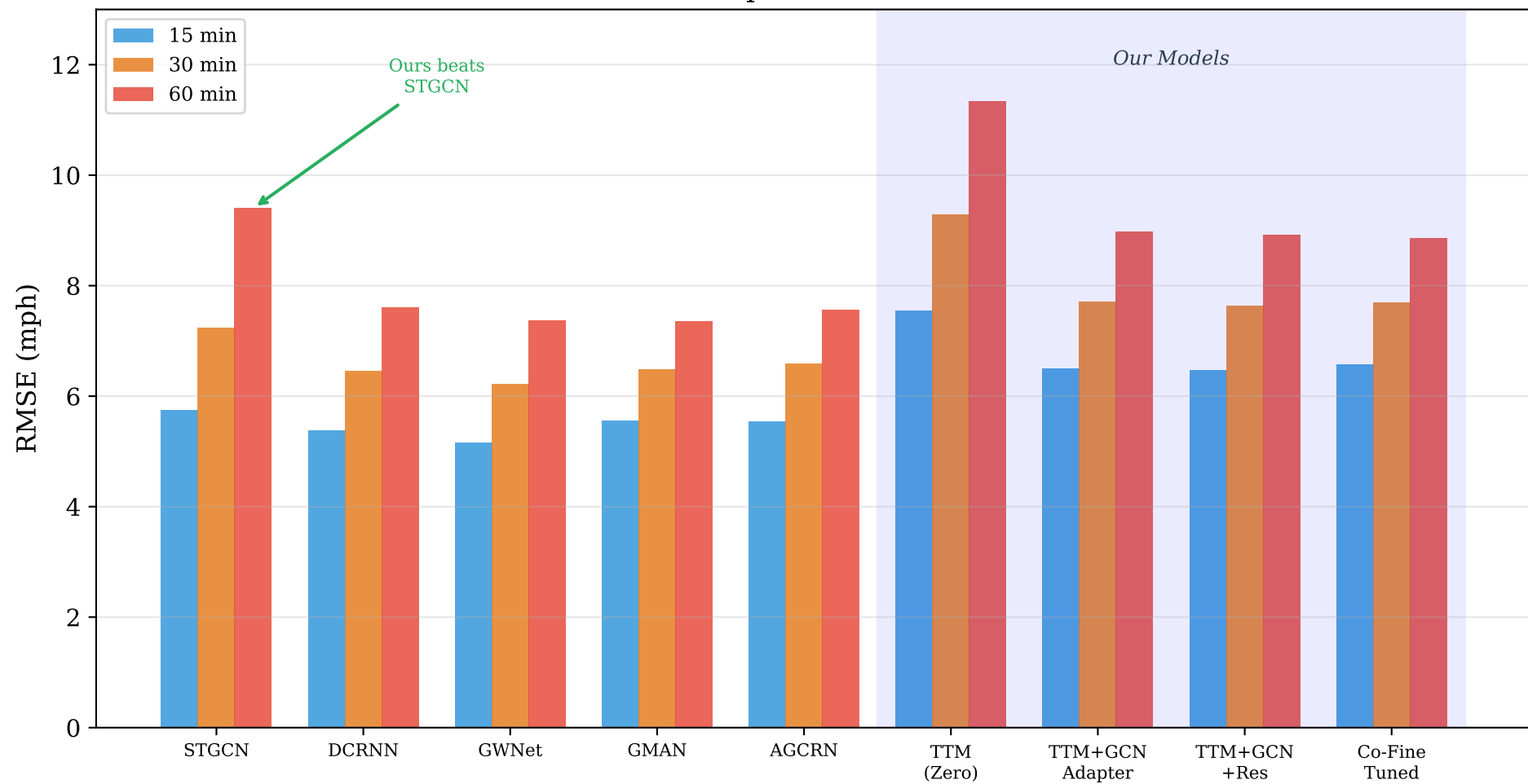
RMSE Comparison on METR-LA
