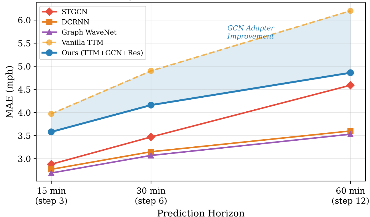
MAE Degradation Across Prediction Horizons
