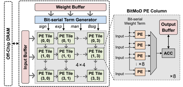
Fig. 6: BitMoD accelerator architecture.
