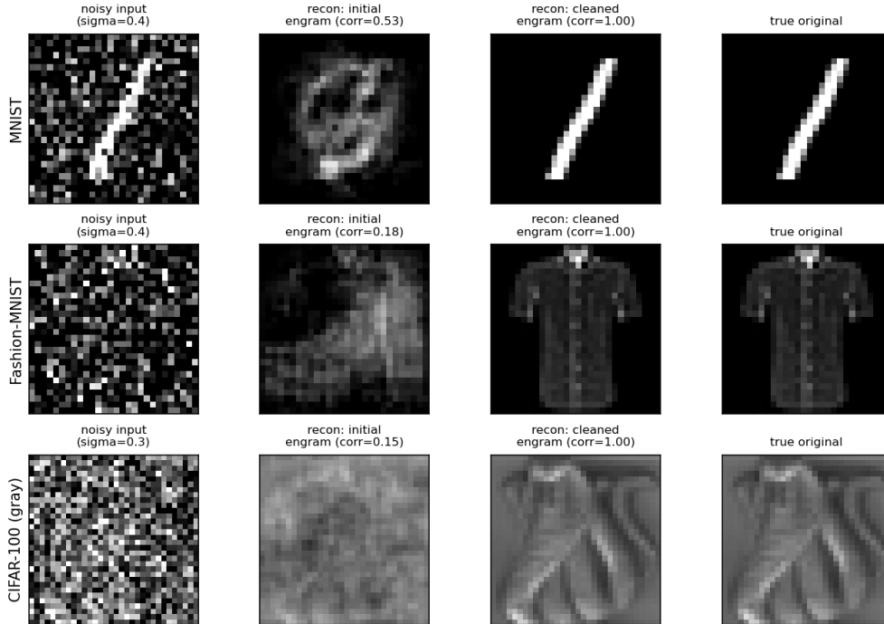
Figure 8: Representative cleanup examples (one dataset per row-group): noisy input, image reconstructed from the engram before cleanup, image reconstructed after the Sudoku-attractor pass, and the true original. All cases shown are exact grid recoveries.
