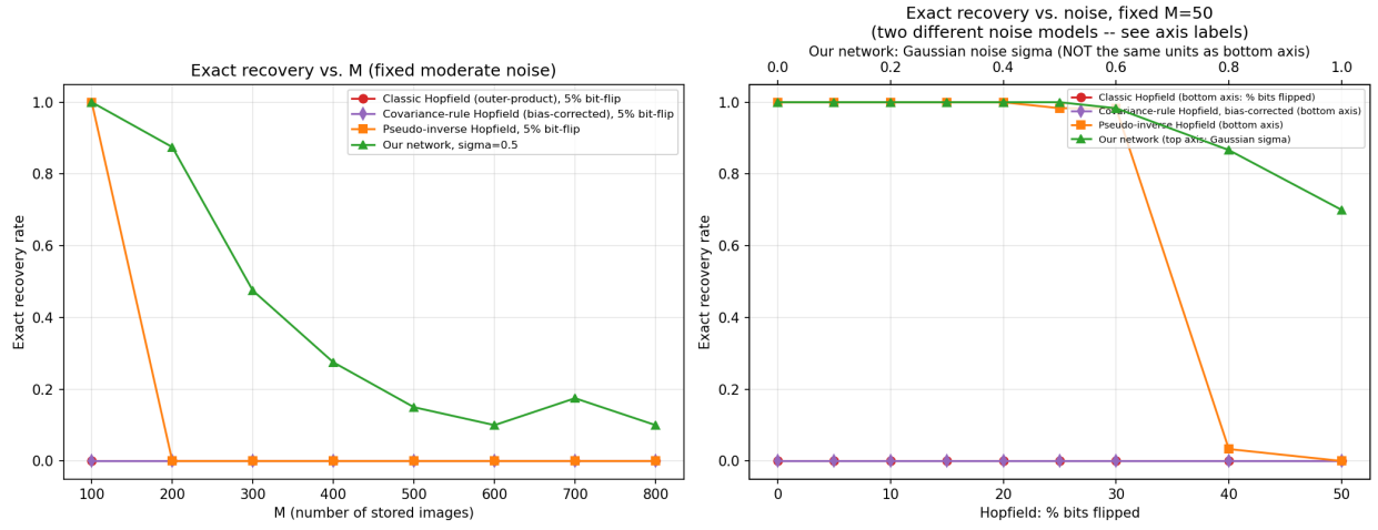
Figure 10: Left: exact recovery vs. M , all four methods, fixed moderate noise. Right: exact recovery vs. noise at fixed M=50 (chosen below every method's zero-noise collapse point), two separate noise axes since the corruption models differ.
