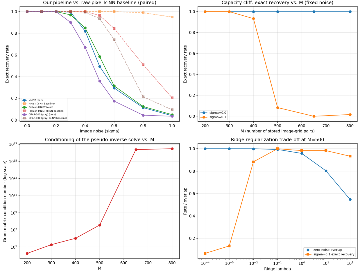
Figure 9: Top-left: our pipeline vs. the nearest-neighbor baseline (paired). Top-right: the M=500 cliff under the default ridge. Bottom-left: image Gram-matrix condition number vs. M (log scale), crossing the ridge value exactly where the cliff appears. Bottom-right: ridge sensitivity at M=500 , showing the fix.
