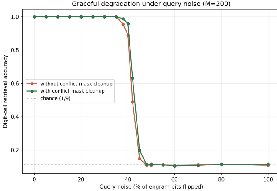
Figure 2: Digit-cell retrieval accuracy vs. query noise, with and without the conflict-mask cleanup pass. Degradation is graceful (a narrow transition window, not a cliff), and cleanup measurably rescues accuracy specifically inside that window.
