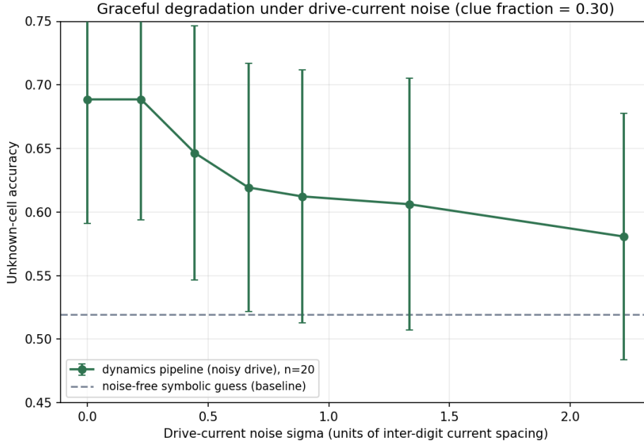
Figure 7: Unknown-cell accuracy vs. Gaussian drive-current noise (clue fraction 0.30), compared against the noise-free symbolic-guess baseline. Degradation is smooth, and the dynamics pipeline stays above baseline throughout the tested range.
