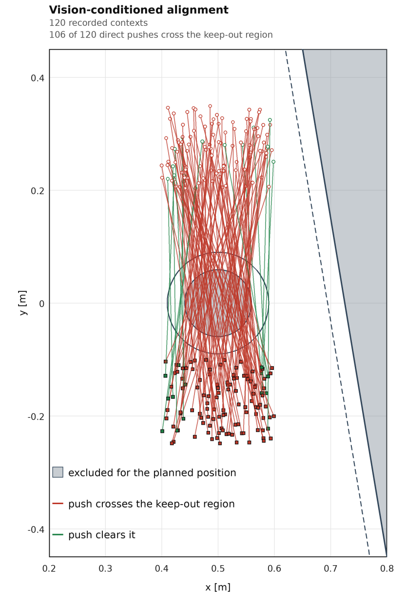
The constraint set and the 120 recorded contexts. Thesis Fig. 5.10
