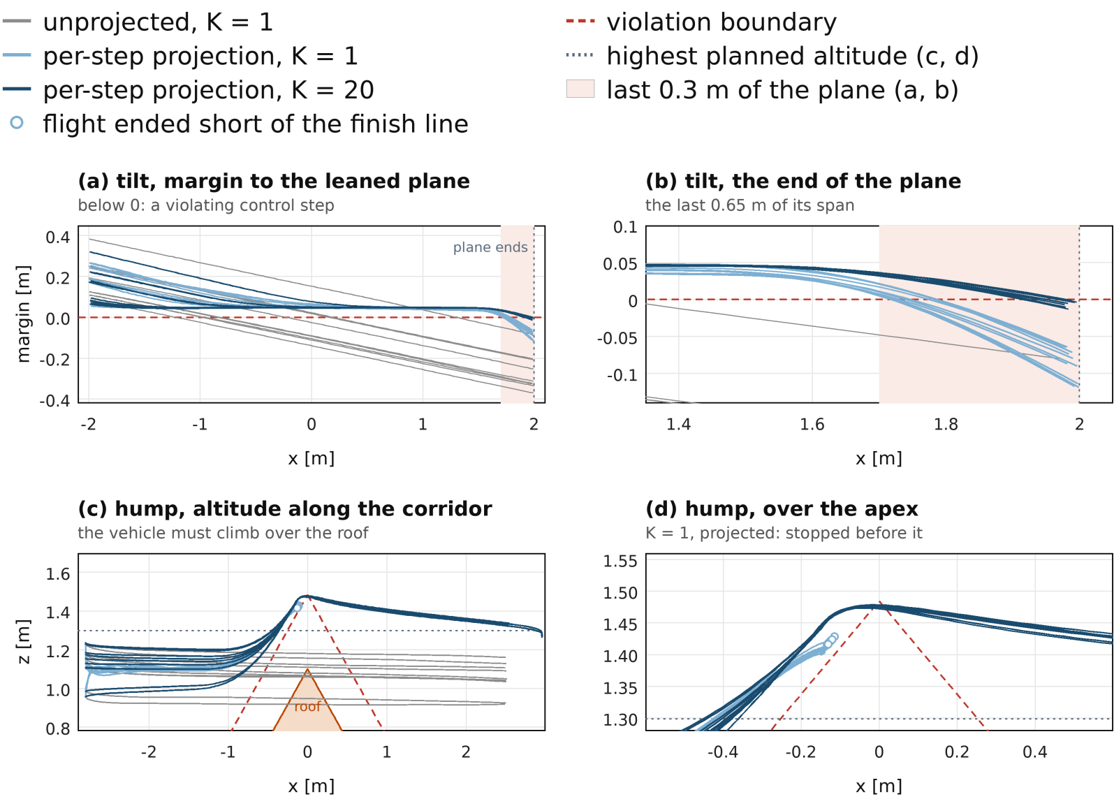
Margin to the tilt and altitude over the hump along the corridor: unprojected, per-step projection at K = 1 and K = 20 ; panel (d): the K = 1 flight stops before the apex. Thesis Fig. B.4
