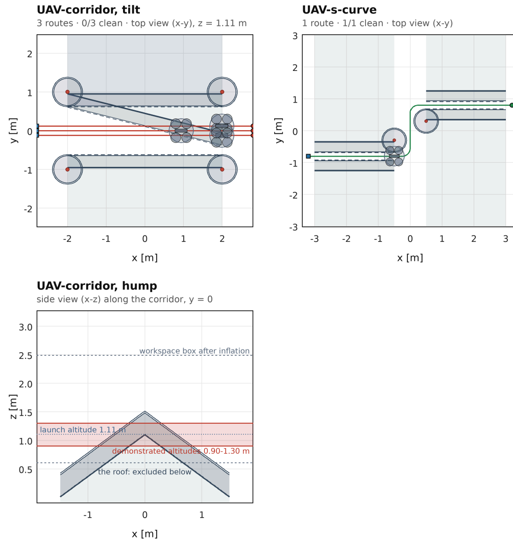
Left: UAV-corridor, the tilt from above and the hump from the side; right: UAV-s-curve. Thesis Fig. 5.11
