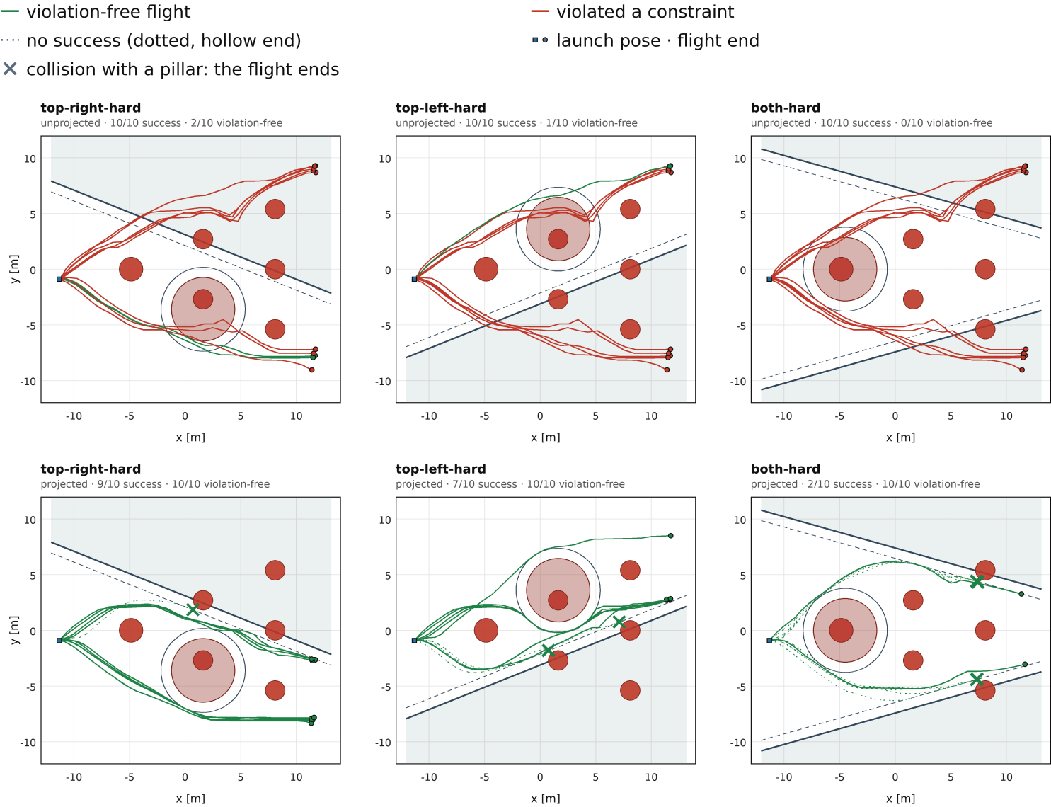
Flown paths, unprojected (top) and projected (bottom), three geometries. Thesis Fig. 6.5
