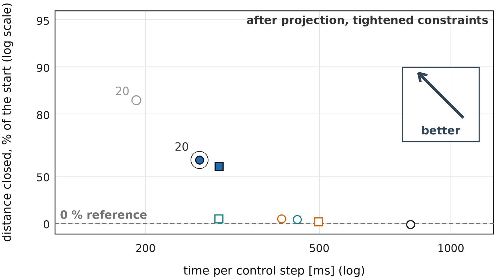
Distance closed against time per control step after projection; circles per-step, squares endpoint; filled points keep at least nine of ten contexts free of violations. Thesis Fig. 6.4
