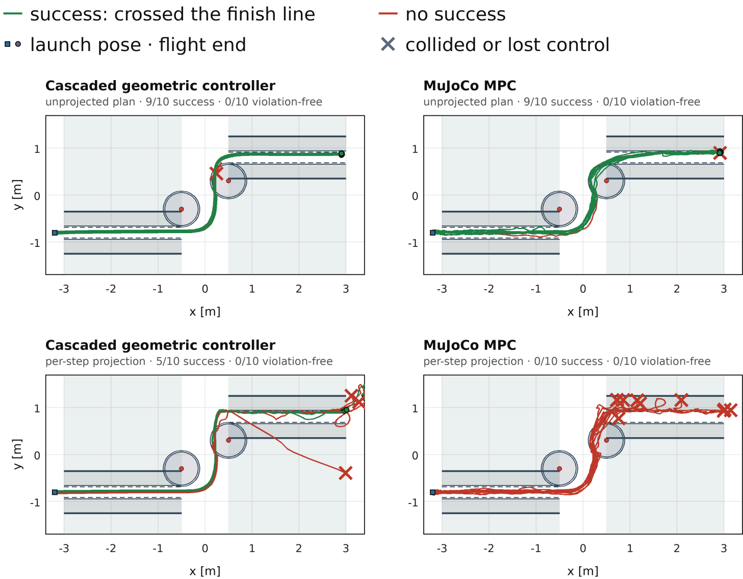
Cascaded geometric controller (left) and MuJoCo MPC (right); unprojected (top) and per-step projection (bottom). Thesis Fig. 6.7
