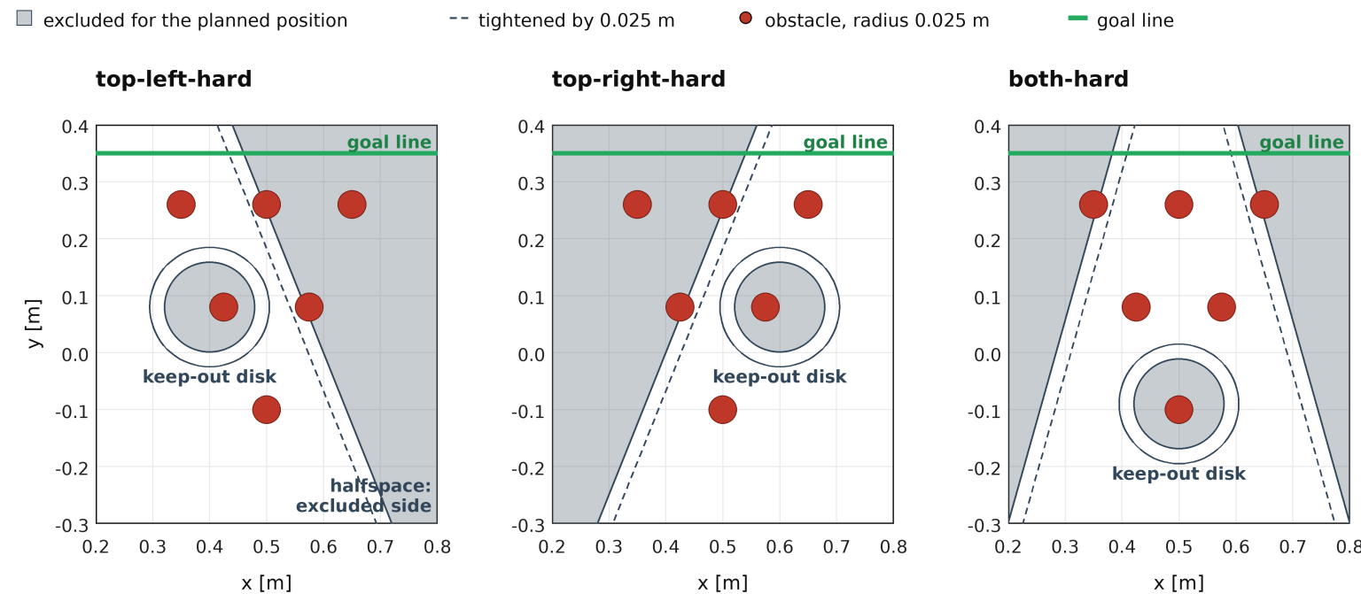
The three constraint geometries of D3IL-avoiding, introduced at test time (thesis figure).
