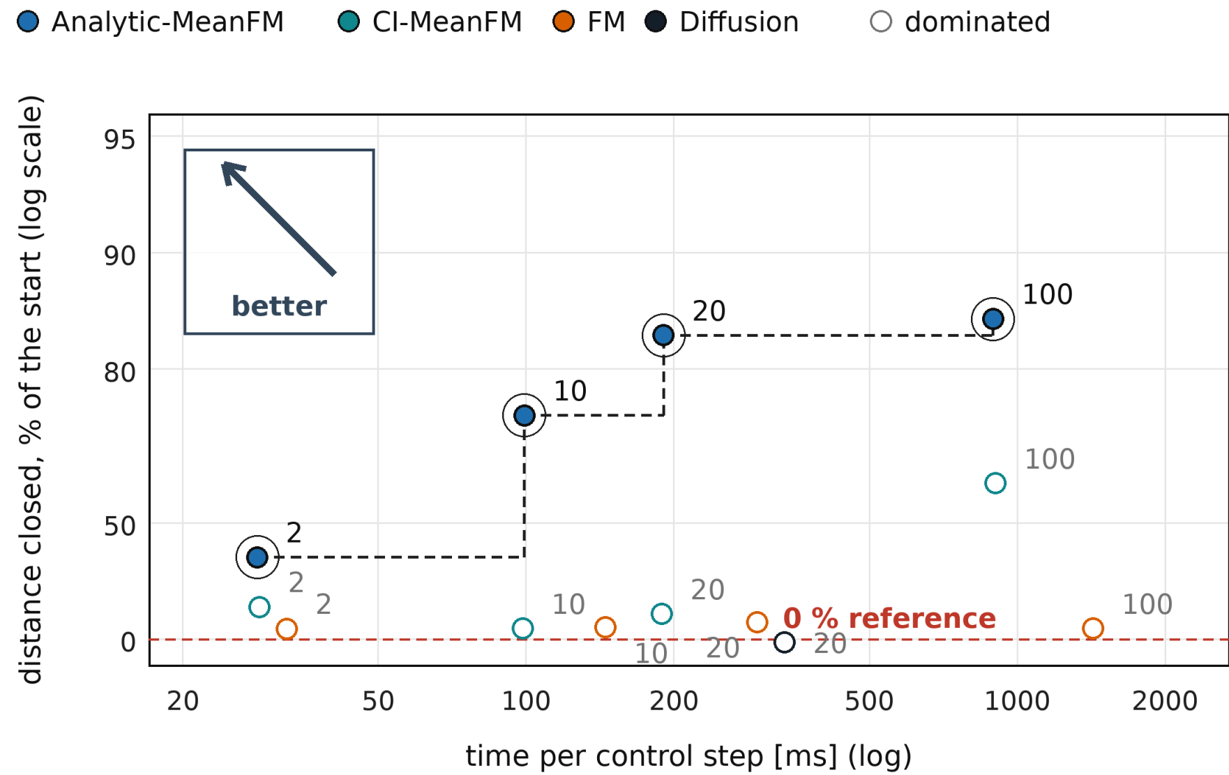
Distance closed against time per control step, every budget, without projection (thesis figure).
