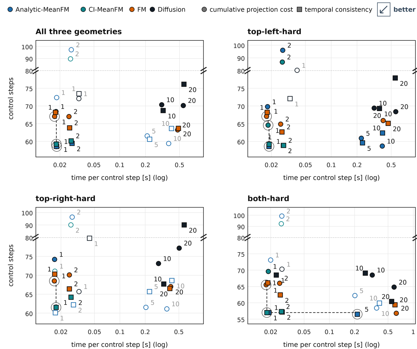
Control steps against time per control step for every budget and selection rule, all three geometries (thesis figure). The talk shows the operating points.
