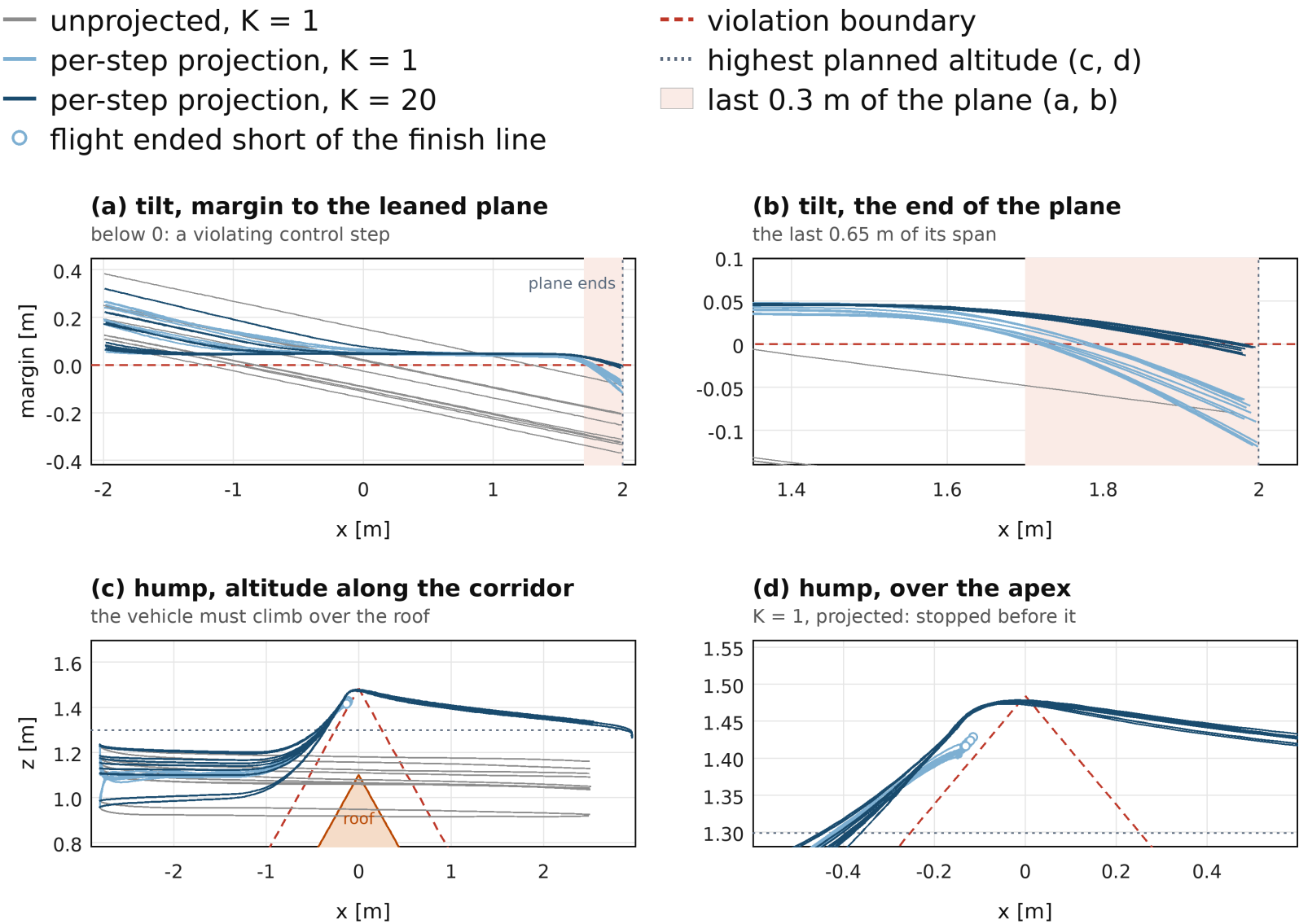
Margin to the tilt and altitude over the hump along the corridor: unprojected, per-step projection at K = 1 and K = 20 (thesis figure). Panel (d): the K = 1 flight stops before the apex.
