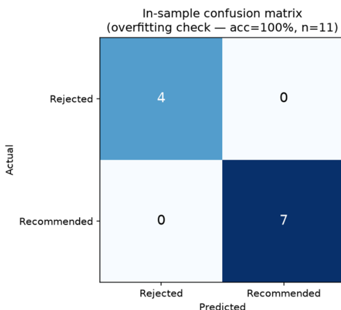
Figure 2a: confusion_matrix.png (in-sample classification results for the n=11 model.)
