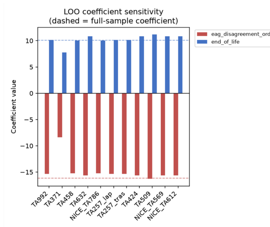
Figure 2b: loo_sensitivity.png (leave-one-out coefficient sensitivity across all 11 refits.)
