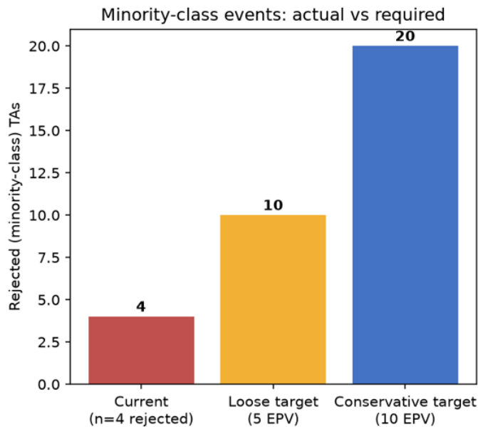
Figure 2c: epv_summary.png (events-per-variable shortfall and implied minimum dataset size.)
