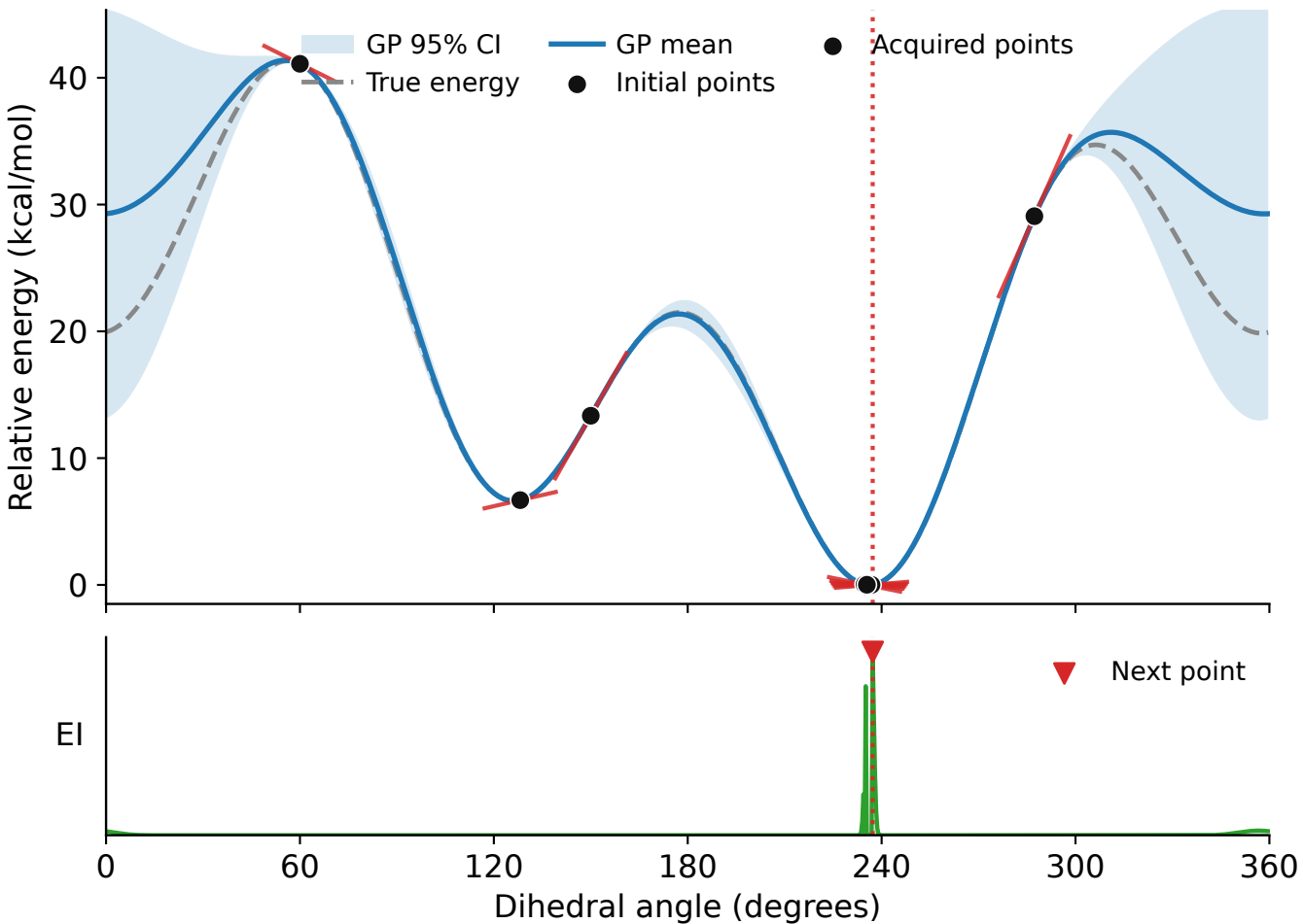
Gradient-enhanced GP — 10 evaluations (best: 0.00 kcal/mol)
