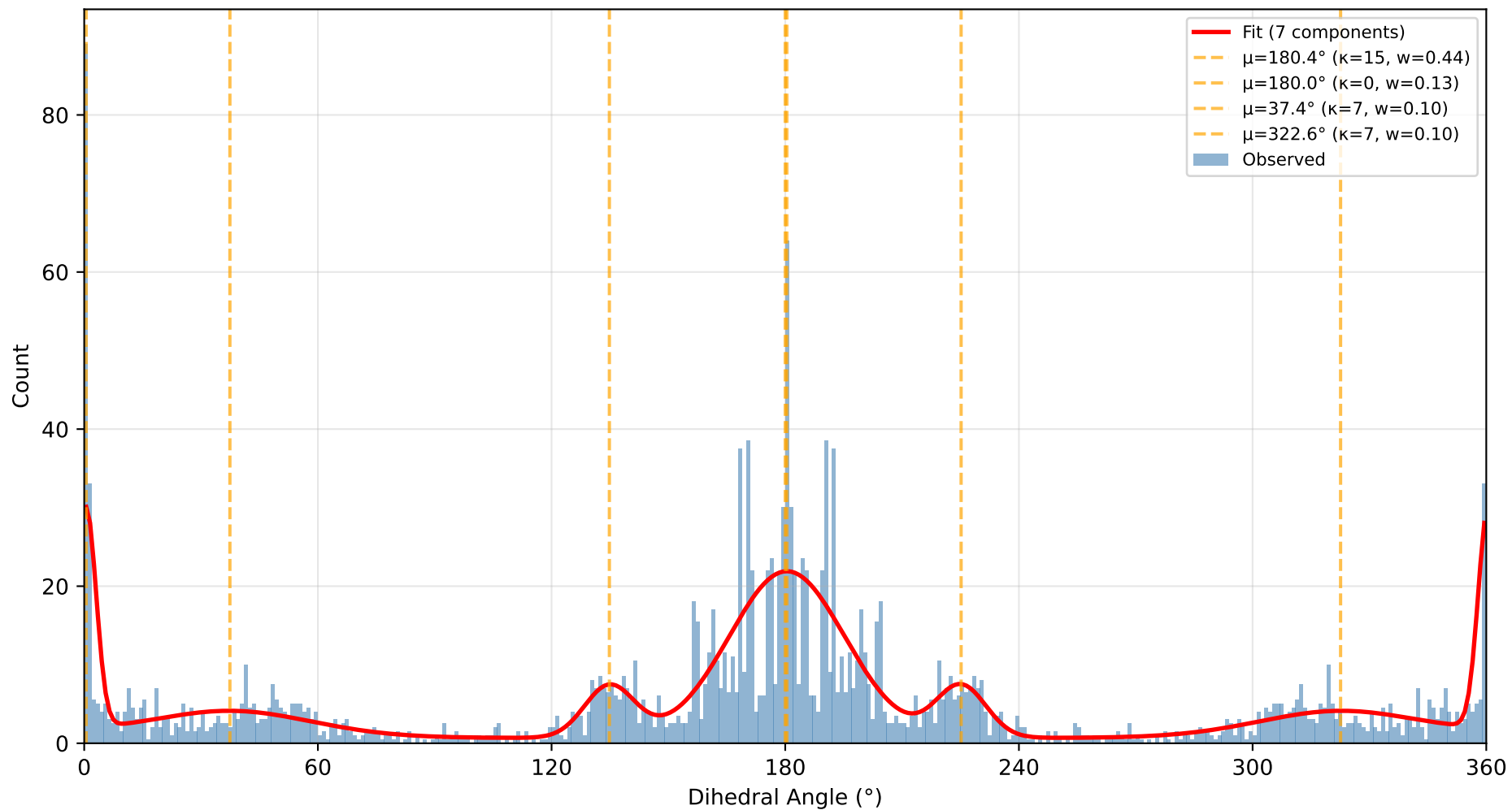
Pattern 217: [cH0:1][c:2]([cH1])!@[c:3]([cH1:4])[cH1] BC=0.9465, RMSE=5.6, n=1,799
