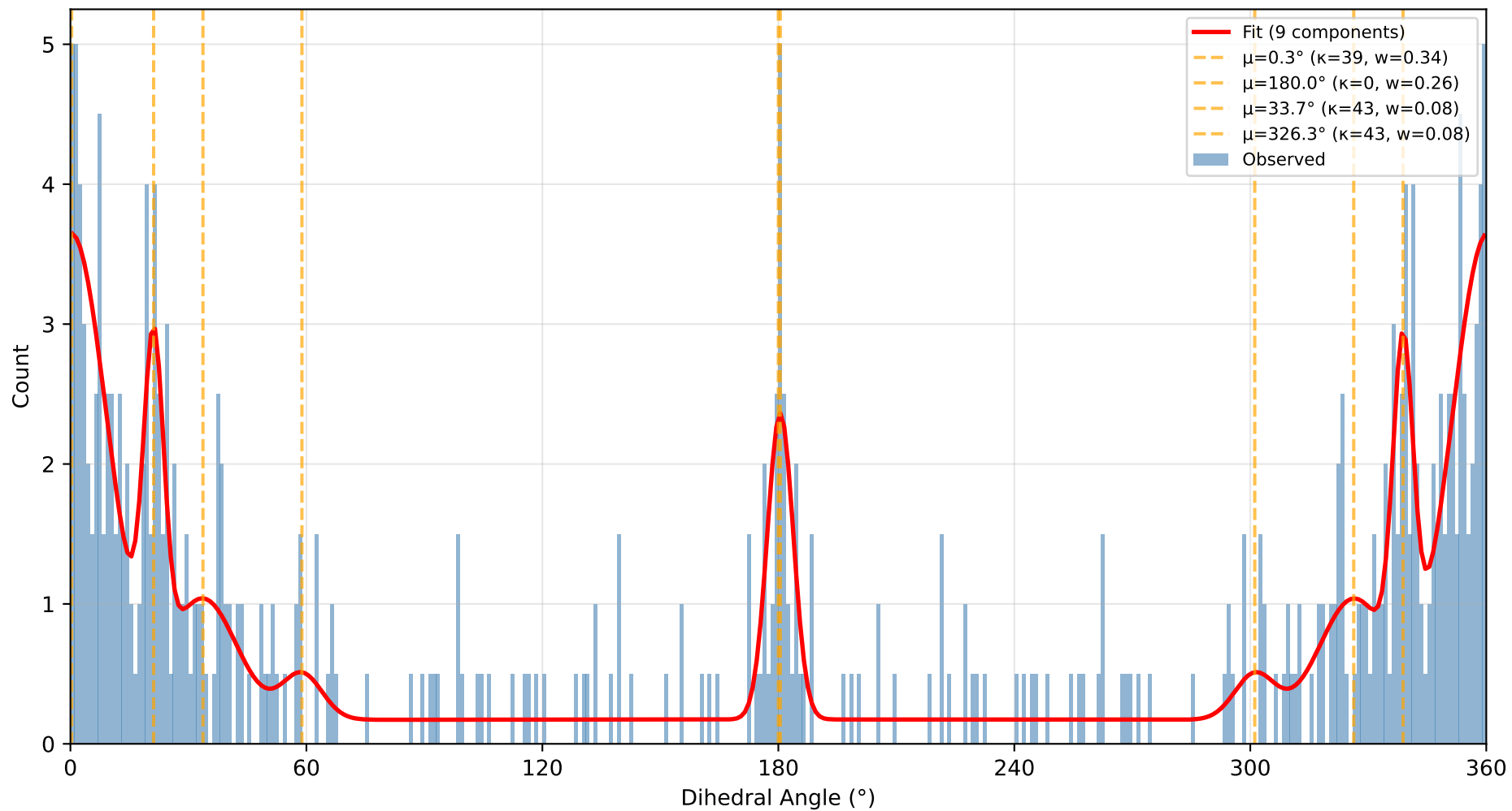
Pattern 377: [$([cH0][OH0]):1][c:2]([cH1])!@[C:3](=O)[NX3H1:4] BC=0.8679, RMSE=0.6, n=235
