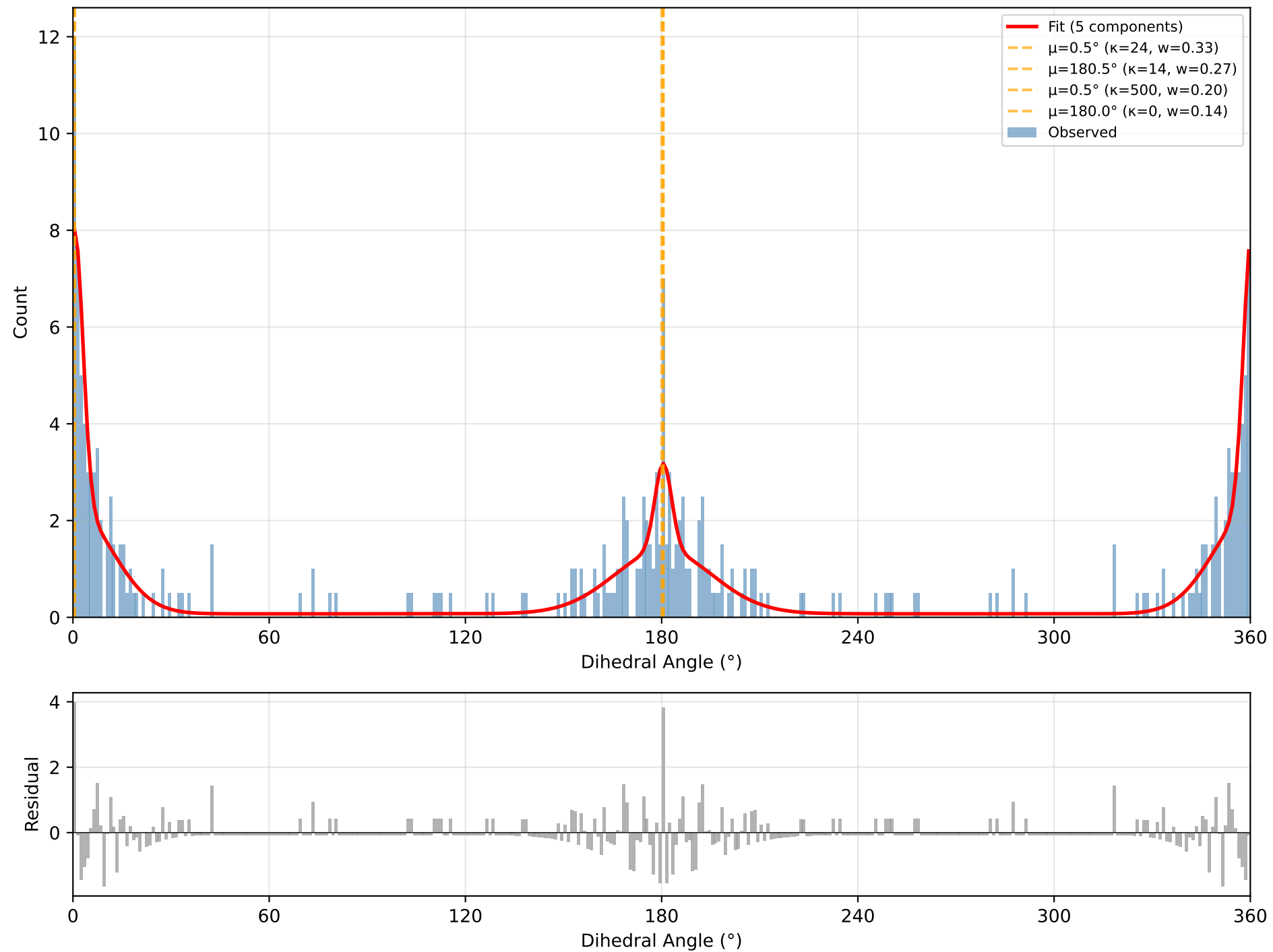
Pattern 378: [$([cH0][OH1]):1][c:2]([cH1])!@[C:3](=O)[NX3H1:4] BC=0.8592, RMSE=0.5, n=187
