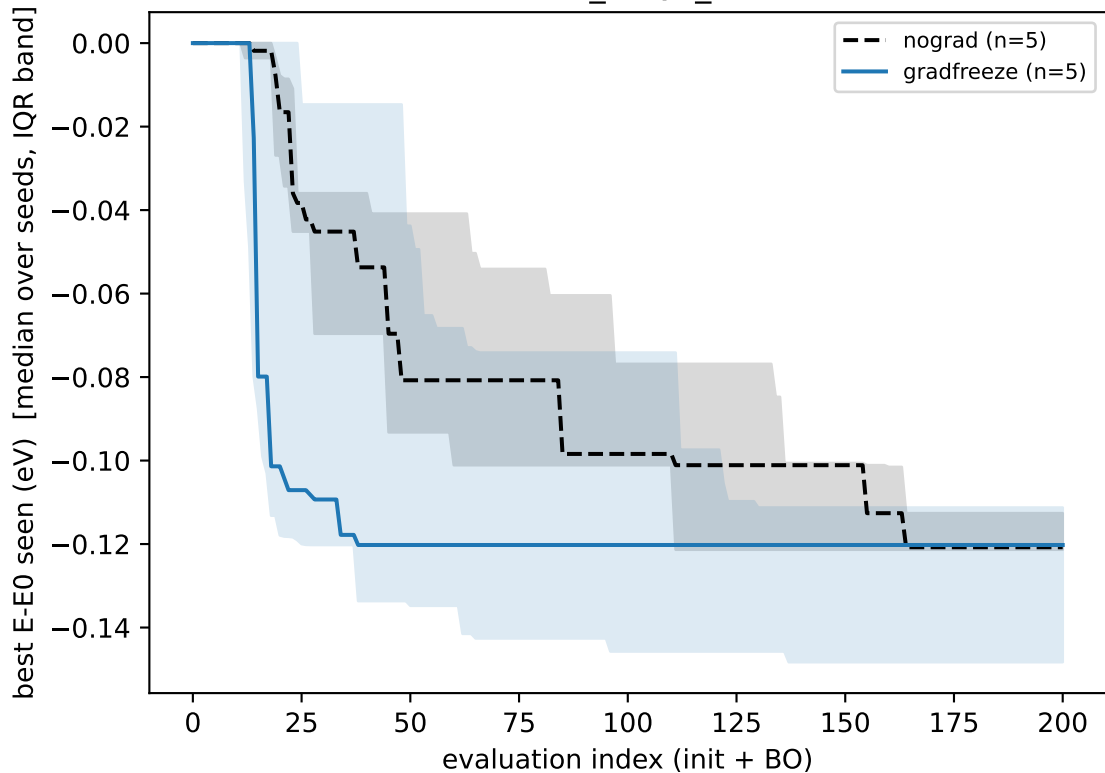
4GZ_4YQD_A
