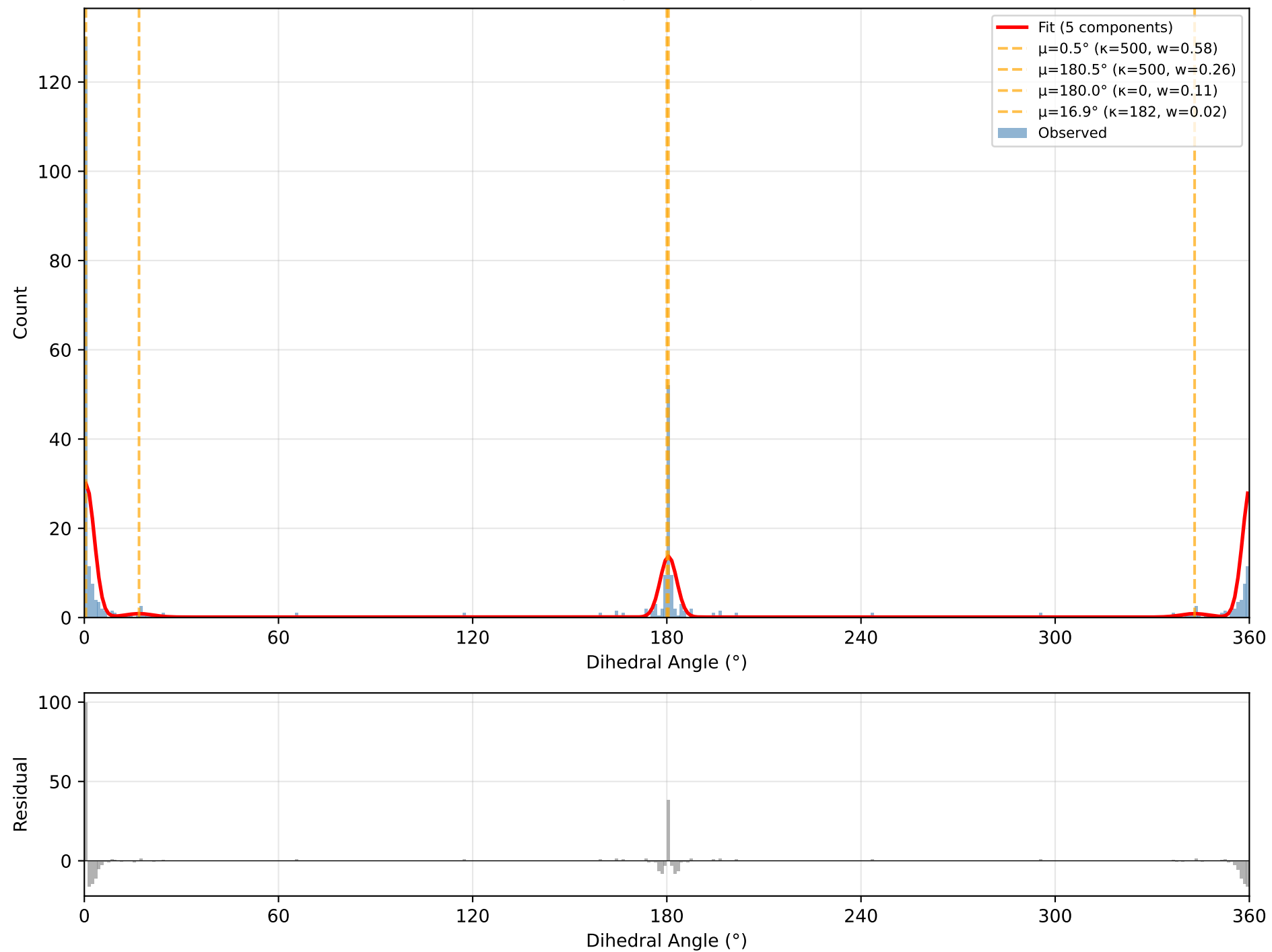
Pattern 219: [nX2H0:1][c:2]!@[c:3][nX3H1:4] BC=0.7945, RMSE=6.0, n=333
