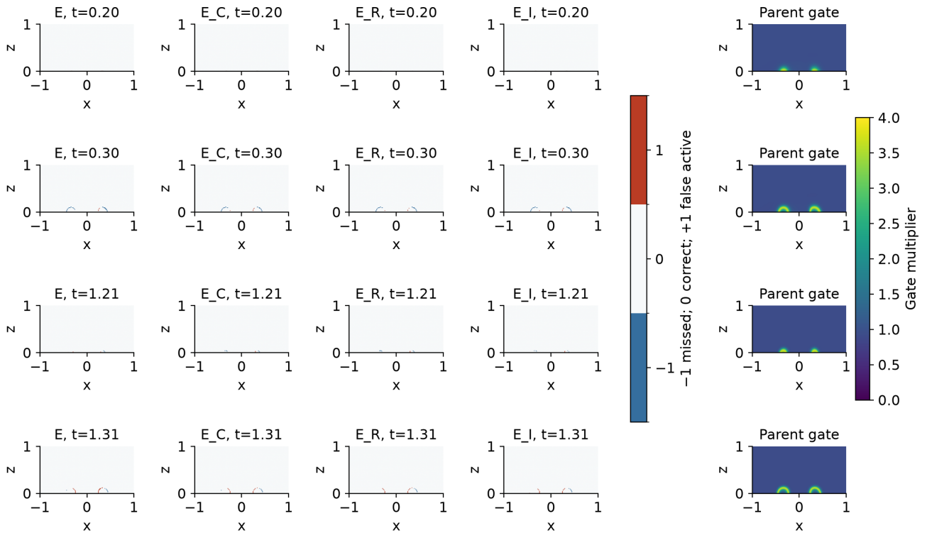
Figure S1. Same complete-domain times, colors and normalization as main Figure 8. The gate depends only on the frozen parent, never on reference error. Complete time traces accompany the portable scores; no favorable crop or time was selected from dense truth.
