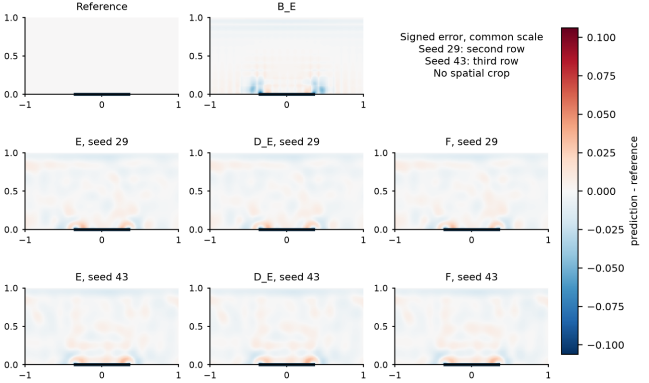
Figure S15. B1 temperature signed prediction-minus-reference error at t=1.28 . Reference, shared B_E and all E/D_E/F states for both seeds are retained. The reference error panel is zero by definition.
