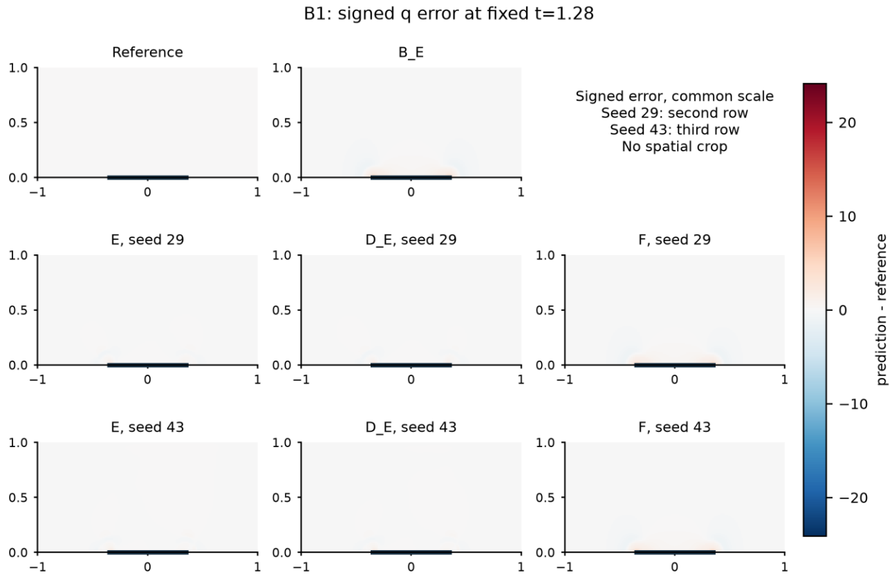
Figure S23. B1 local Joule density signed prediction-minus-reference error at t=1.28. Reference, shared B_E and all E/D_E/F states for both seeds are retained. The reference error panel is zero by definition.
