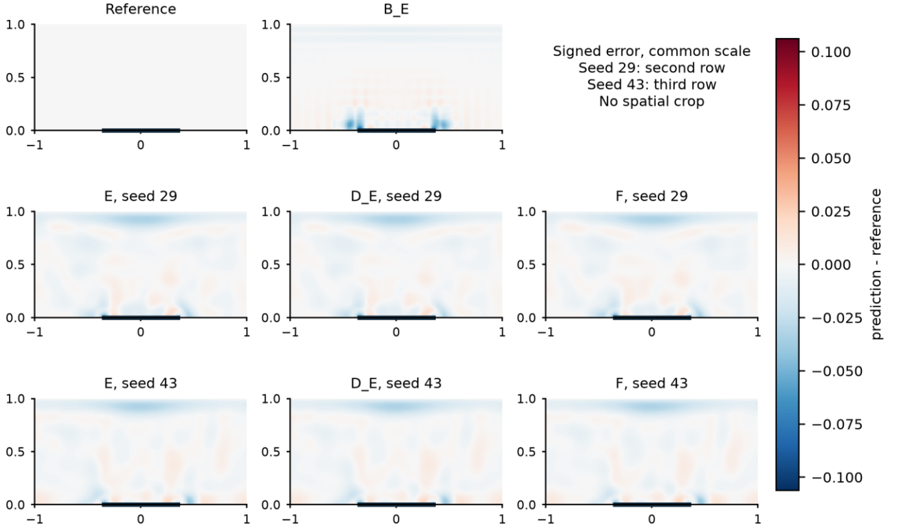
Figure S13. B1 temperature signed prediction-minus-reference error at t=0.27 . Reference, shared B_E and all E/D_E/F states for both seeds are retained. The reference error panel is zero by definition.
