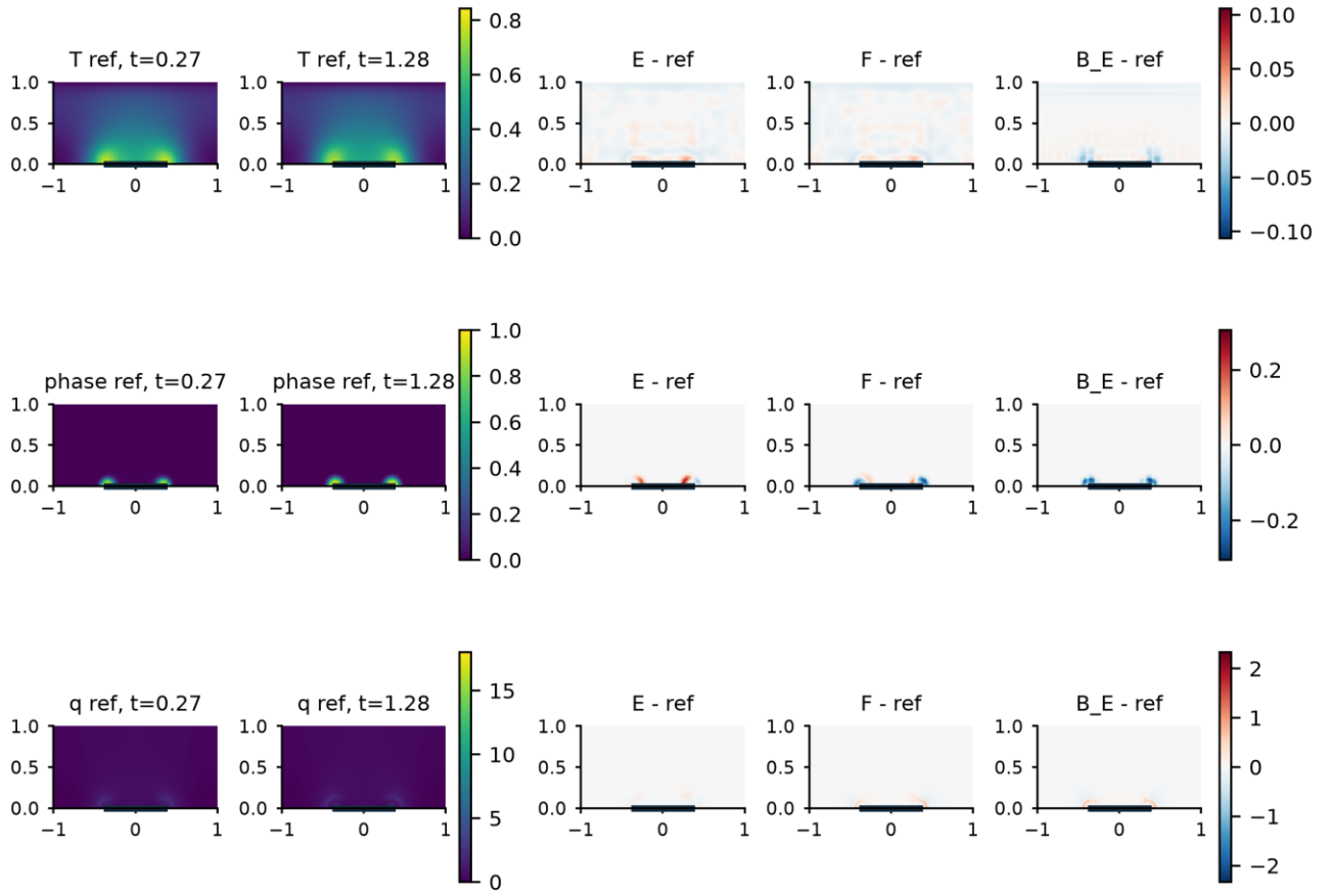
Figure S11. Full-label seed-43 companion to main Figure 2, with the same reference fields, times and signed-error color ranges.
