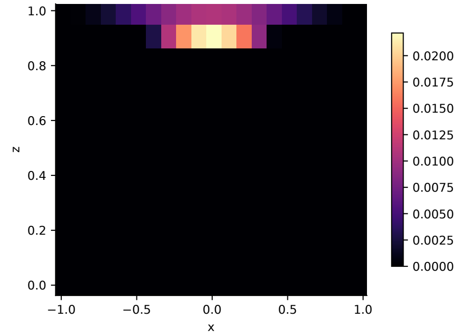
Remaining voltage-error distribution
