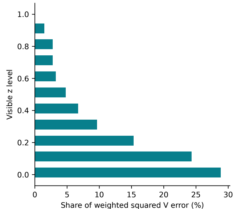
Remaining voltage-error distribution
