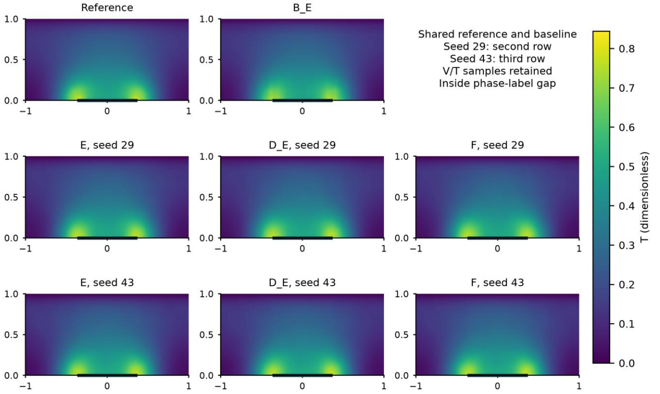
Figure S14. B1 temperature state at t=1.28 . Reference, shared B_E and all E/D_E/F states for both seeds are retained.
