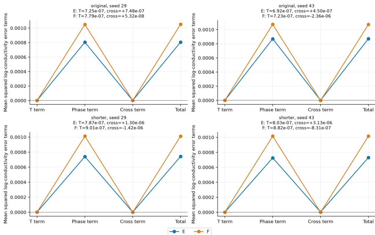
Figure S9. Squared-error terms of the exact log-conductivity identity: temperature, phase, signed cross term and total. Panel annotations retain the small temperature and signed cross values that are difficult to resolve on the common linear axis. The cross term permits cancellation. Neither marginal term is an isolated causal contribution to terminal error, and the identity is not a residual-weighting prescription.
