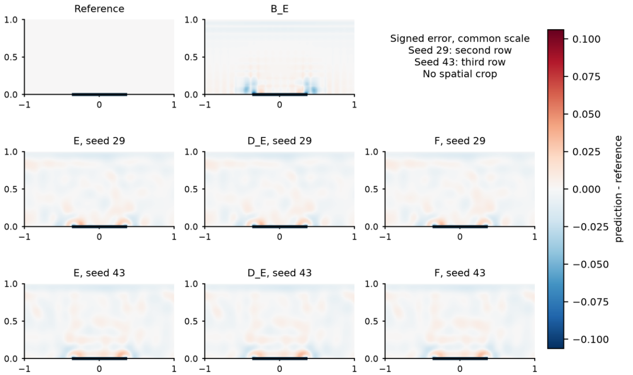
Figure S15. B1 temperature signed prediction-minus-reference error at t=1.28 . Reference, shared B_E and all E/D_E/F states for both seeds are retained. The reference error panel is zero by definition.
