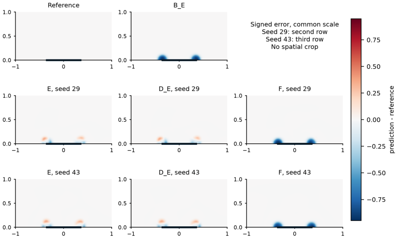
Figure S19. B1 phase signed prediction-minus-reference error at t=1.28 . Reference, shared B_E and all E/D_E/F states for both seeds are retained. The reference error panel is zero by definition.
