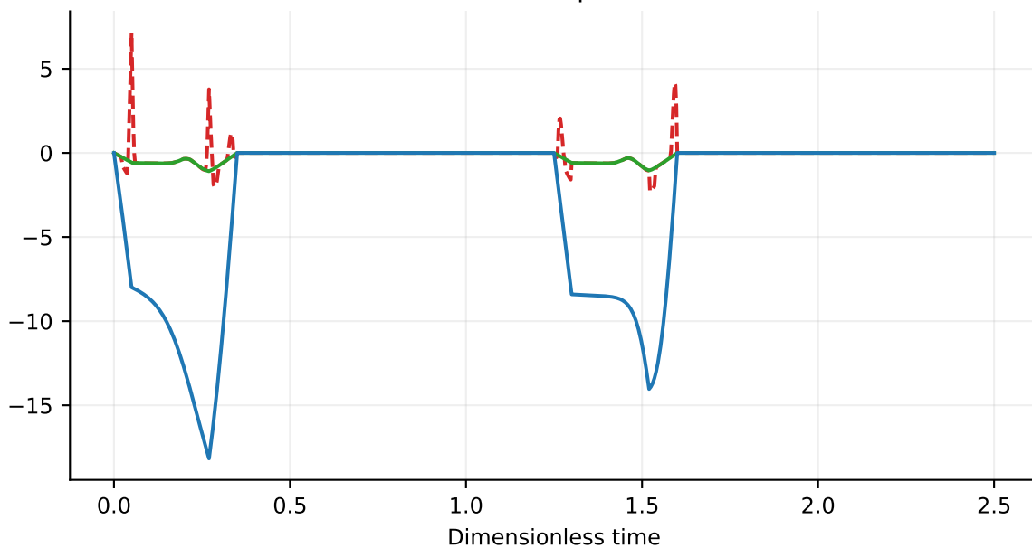
Current balance: top minus bottom
