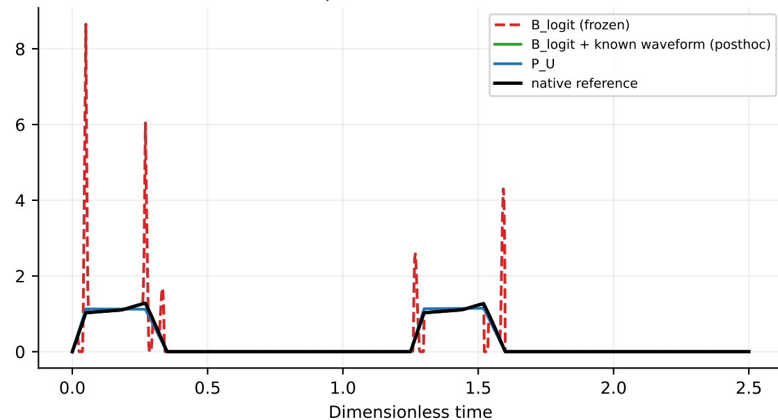
Current balance: top minus bottom
