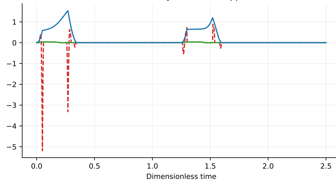
Power defect: Joule minus supplied
