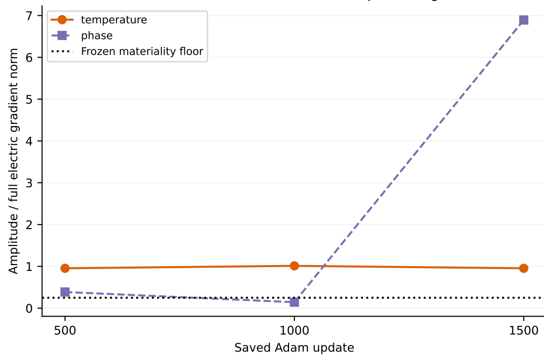
Norm ratios are not contribution percentages
