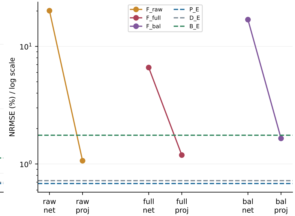
Same learned state: power repair
