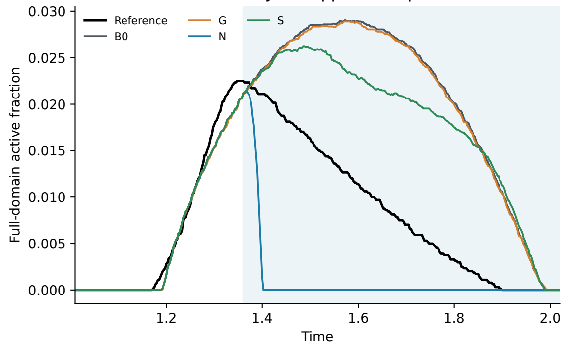
(c) Second-cycle support, complete W
