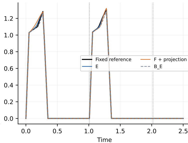
Seed 43: Electrode current
