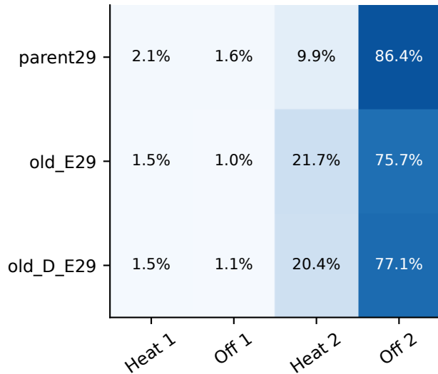
Full logit
