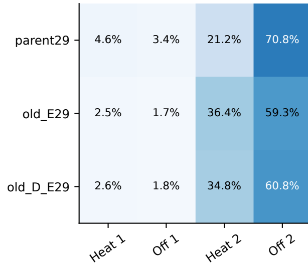
Finite logit
