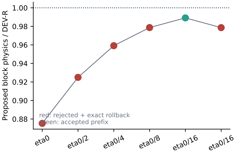
A Identity-correct block screen
