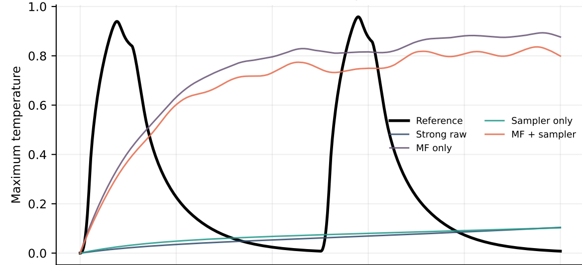
(b) Thermal response
