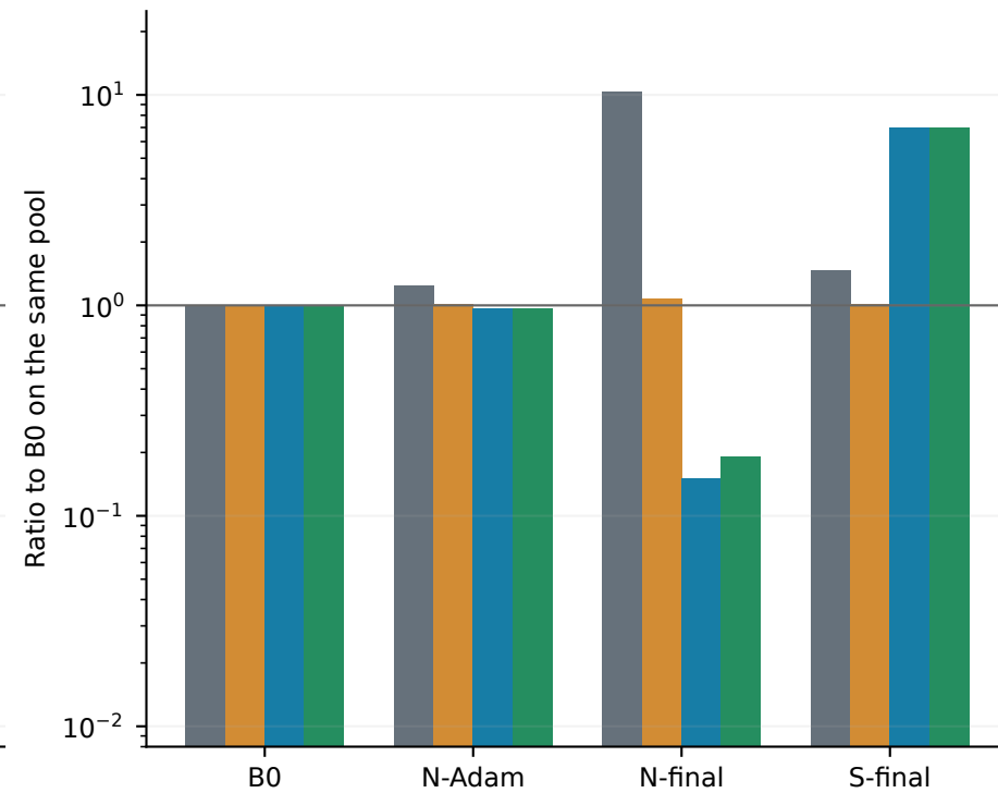
S: bottom-boundary hotspots and coverage
