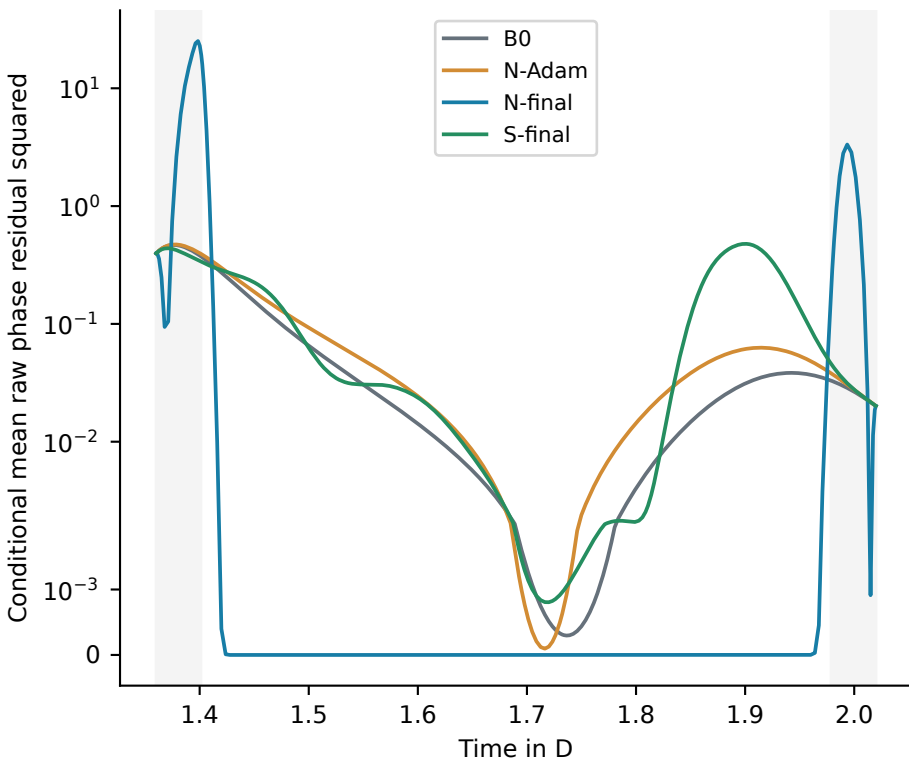
Temporal concentration: same cells and weights
