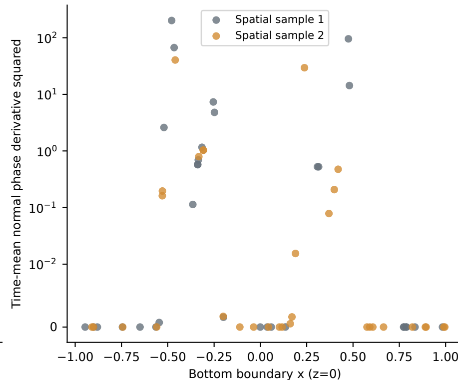
S: bottom-boundary hotspots and coverage
