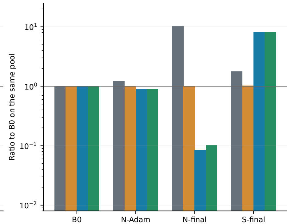
Fixed T: conditional heat identity, 64 cells
