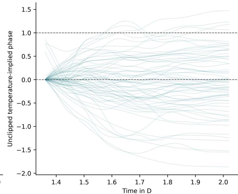
Fixed T: conditional heat identity, 64 cells
