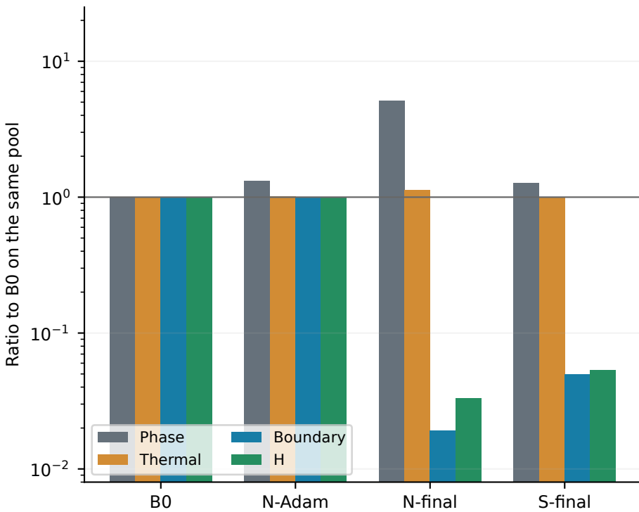
Temporal concentration: same cells and weights
