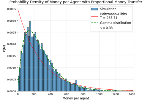
Figure 4: The histogram shows the money distribution of agents after 10^6 number of transactions, while the green line represents the theoretical Gamma distribution and the red line represents the Boltzmann-Gibbs distribution with such temperature. The simulation was performed with N = 3500 , M = 10000 , and \gamma = 1/3 . Agents in this scenario can exchange only a fraction of their money, determined by the saving propensity \gamma .
