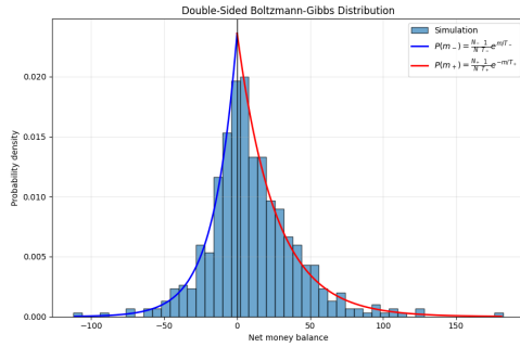
Figure 3: The histogram shows the money distribution of agents after a 10^7 number of transactions, while the red and blue lines represent the theoretical double-sided Boltzmann-Gibbs distribution. The simulation was performed with N = 500 , M = 5000 , and \Delta m = 1 . The reverse ratio is set to r = 0.618 so that the two branches of the distribution meet at the origin.
