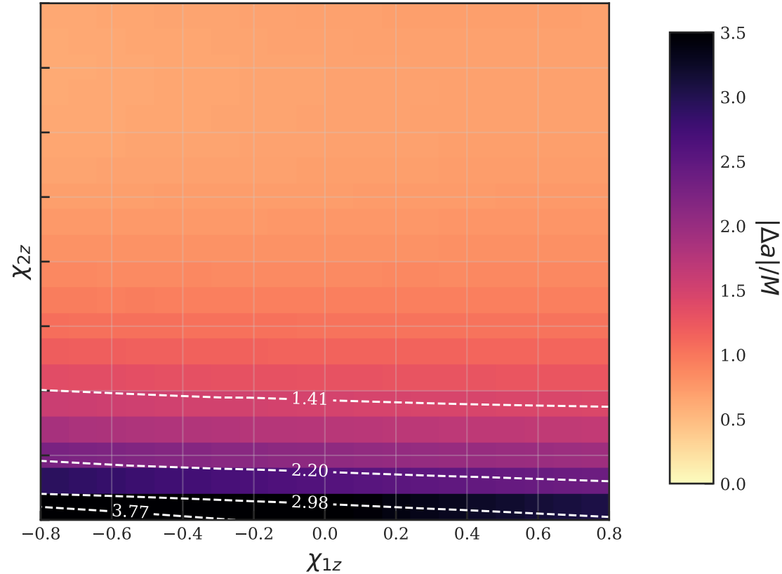
Taylor 2PN
