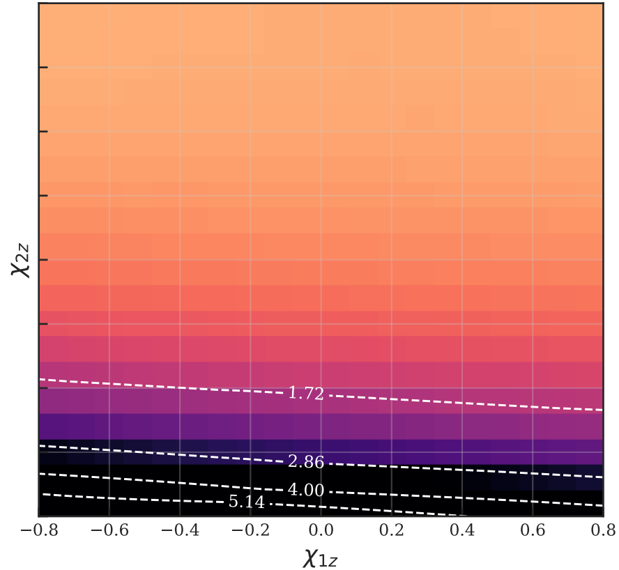
Taylor 1PN
