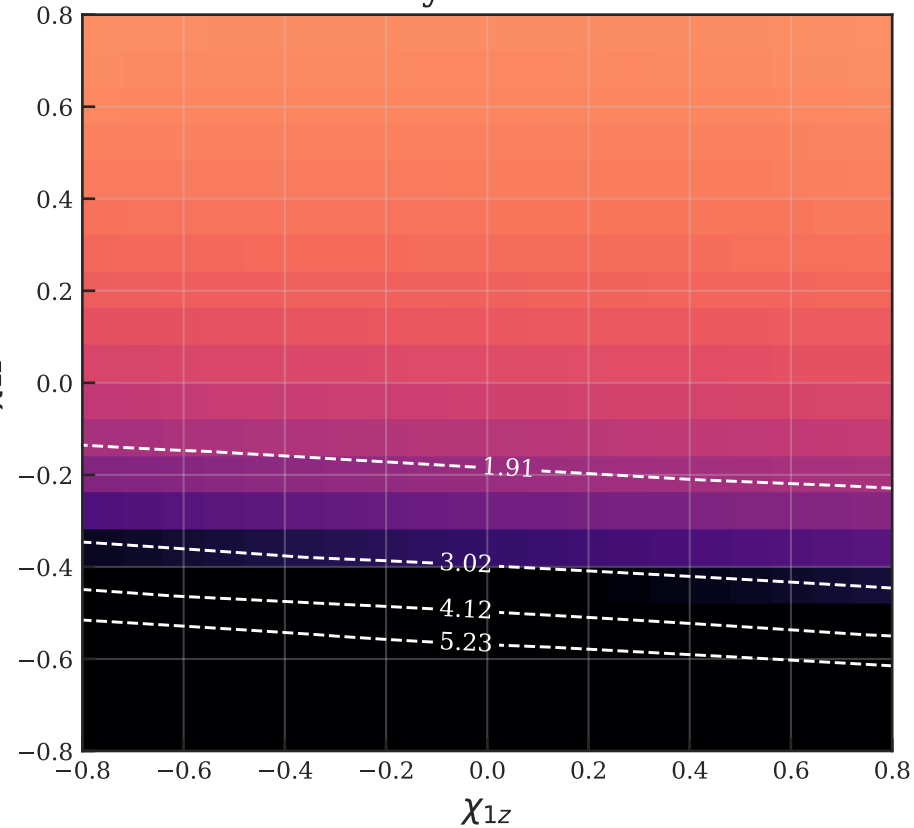
Taylor 0PN
