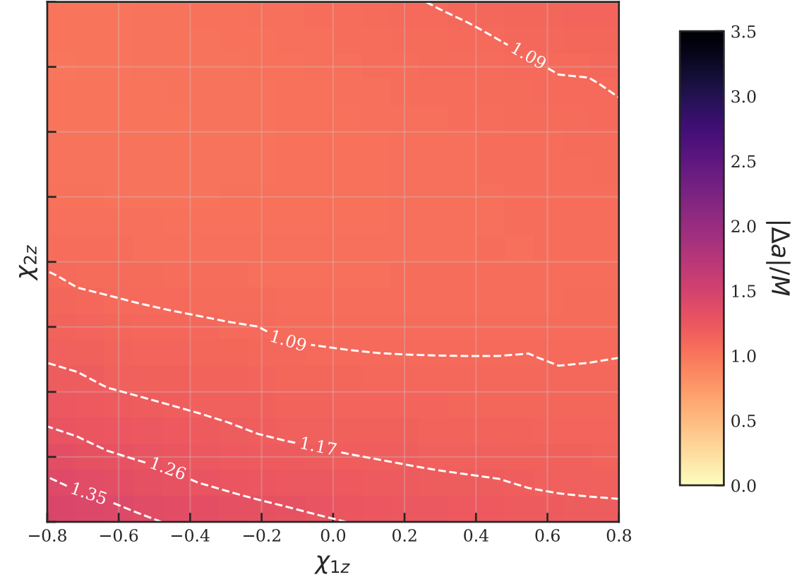
Taylor 2PN
