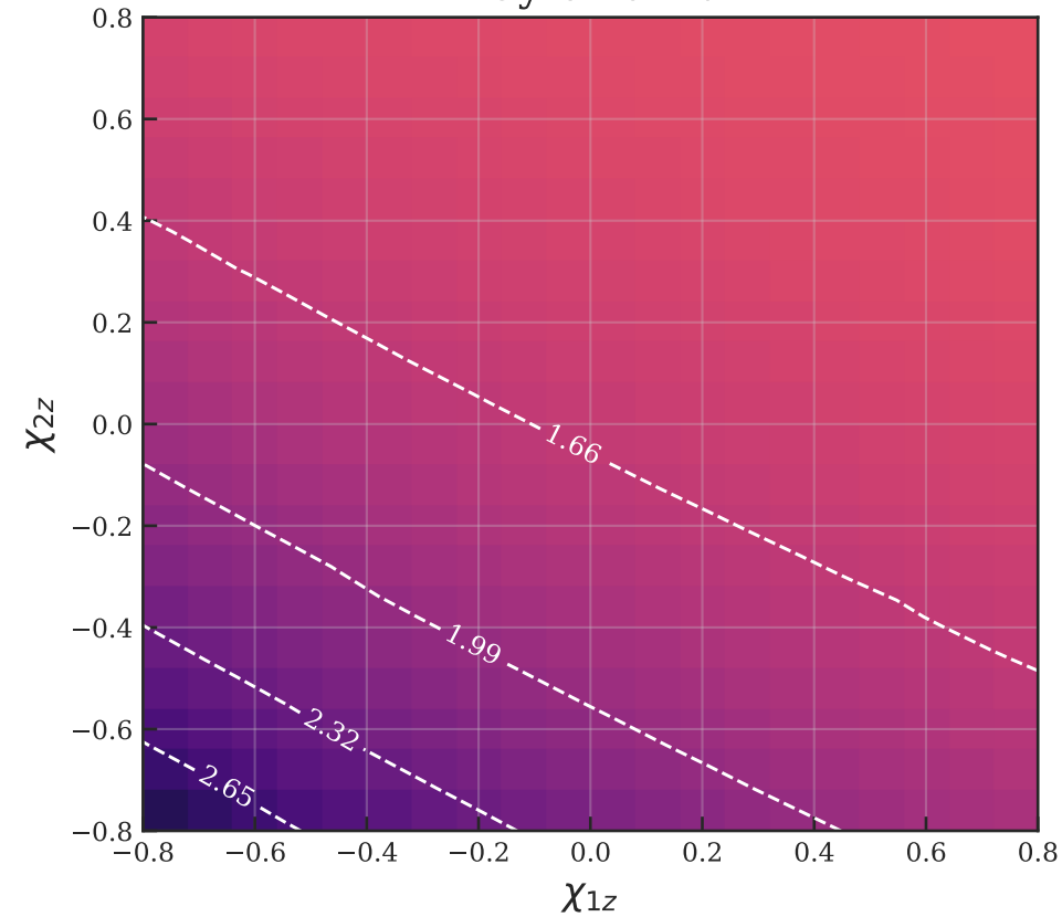
Taylor 0PN
