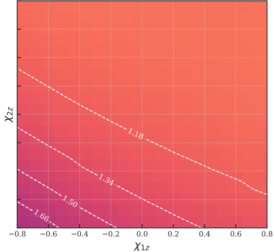
Taylor 1PN
