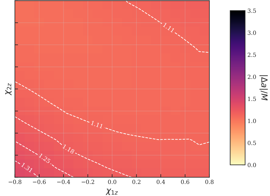
Taylor 2PN
