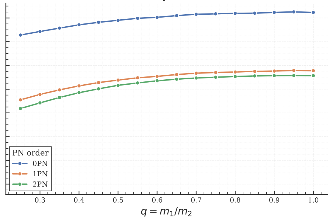
Taylor
